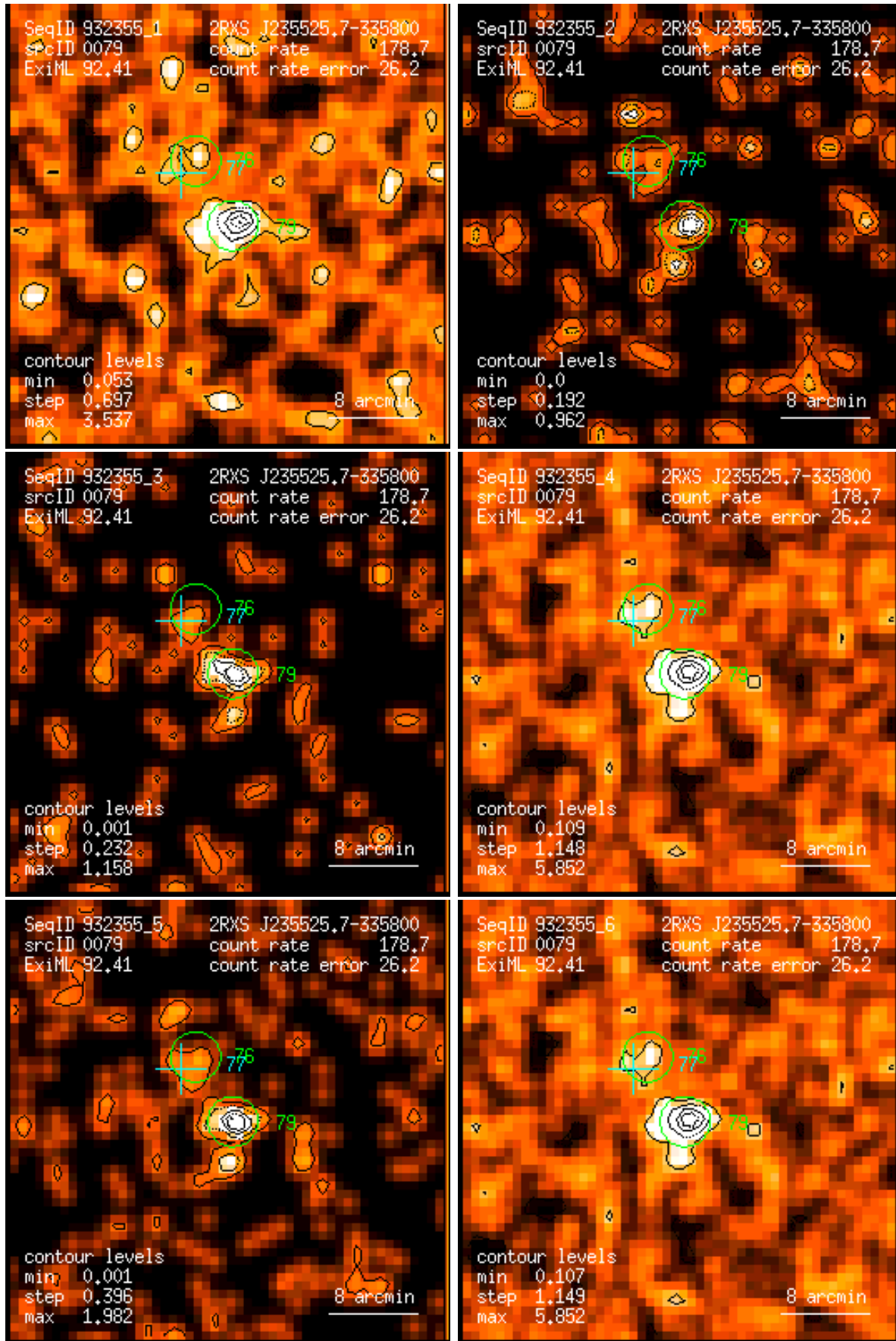
Figure 79: RASS 932355: detection 0079: band rate images, Gaussian filter: (1) PSPC channels 11 – 41, (2) 52 – 90, (3) 91 – 201, (4) 11 – 235, (5) 52 – 201, (6) 11 – 201. Broad band rates in counts/ks. Band rate contour levels in counts/ks/arcmin 2 .
