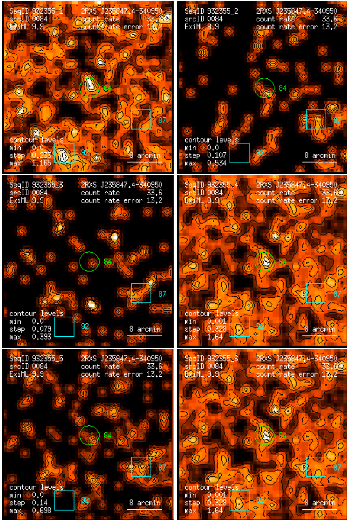
Figure 84: RASS 932355: detection 0084: band rate images, Gaussian filter: (1) PSPC channels 11 – 41, (2) 52 – 90, (3) 91 – 201, (4) 11 – 235, (5) 52 – 201, (6) 11 – 201. Broad band rates in counts/ks. Band rate contour levels in counts/ks/arcmin 2 .
