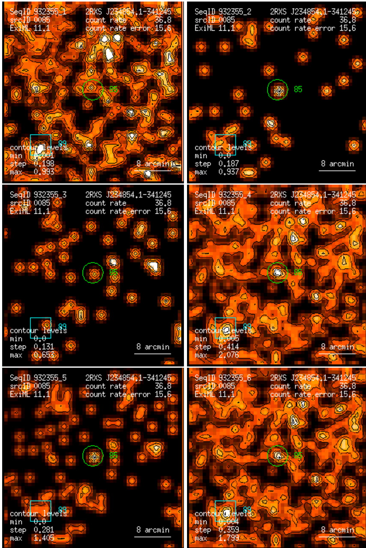
Figure 85: RASS 932355: detection 0085: band rate images, Gaussian filter: (1) PSPC channels 11 – 41, (2) 52 – 90, (3) 91 – 201, (4) 11 – 235, (5) 52 – 201, (6) 11 – 201. Broad band rates in counts/ks. Band rate contour levels in counts/ks/arcmin 2 .
