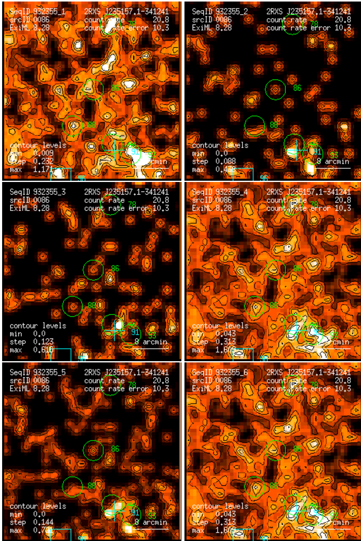
Figure 86: RASS 932355: detection 0086: band rate images, Gaussian filter: (1) PSPC channels 11 – 41, (2) 52 – 90, (3) 91 – 201, (4) 11 – 235, (5) 52 – 201, (6) 11 – 201. Broad band rates in counts/ks. Band rate contour levels in counts/ks/arcmin 2 .
