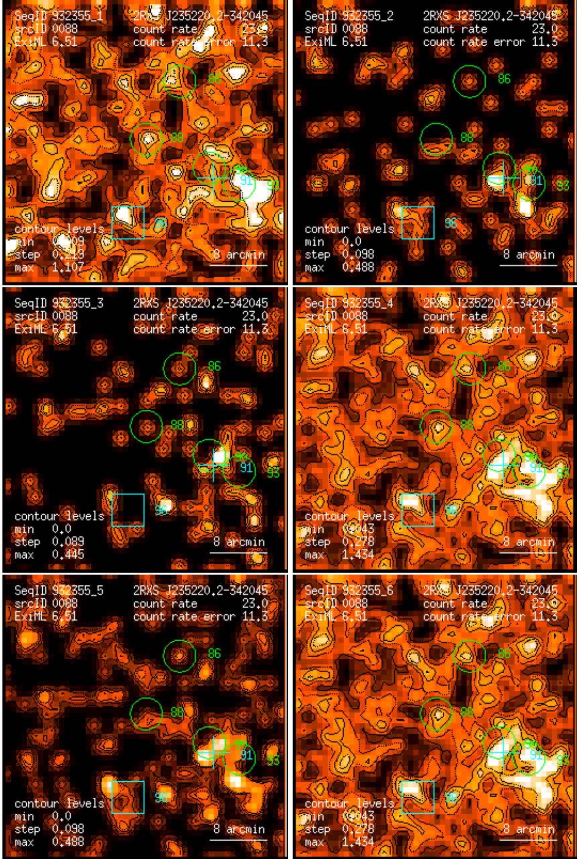
Figure 88: RASS 932355: detection 0088: band rate images, Gaussian filter: (1) PSPC channels 11 – 41, (2) 52 – 90, (3) 91 – 201, (4) 11 – 235, (5) 52 – 201, (6) 11 – 201. Broad band rates in counts/ks. Band rate contour levels in counts/ks/arcmin 2 .
