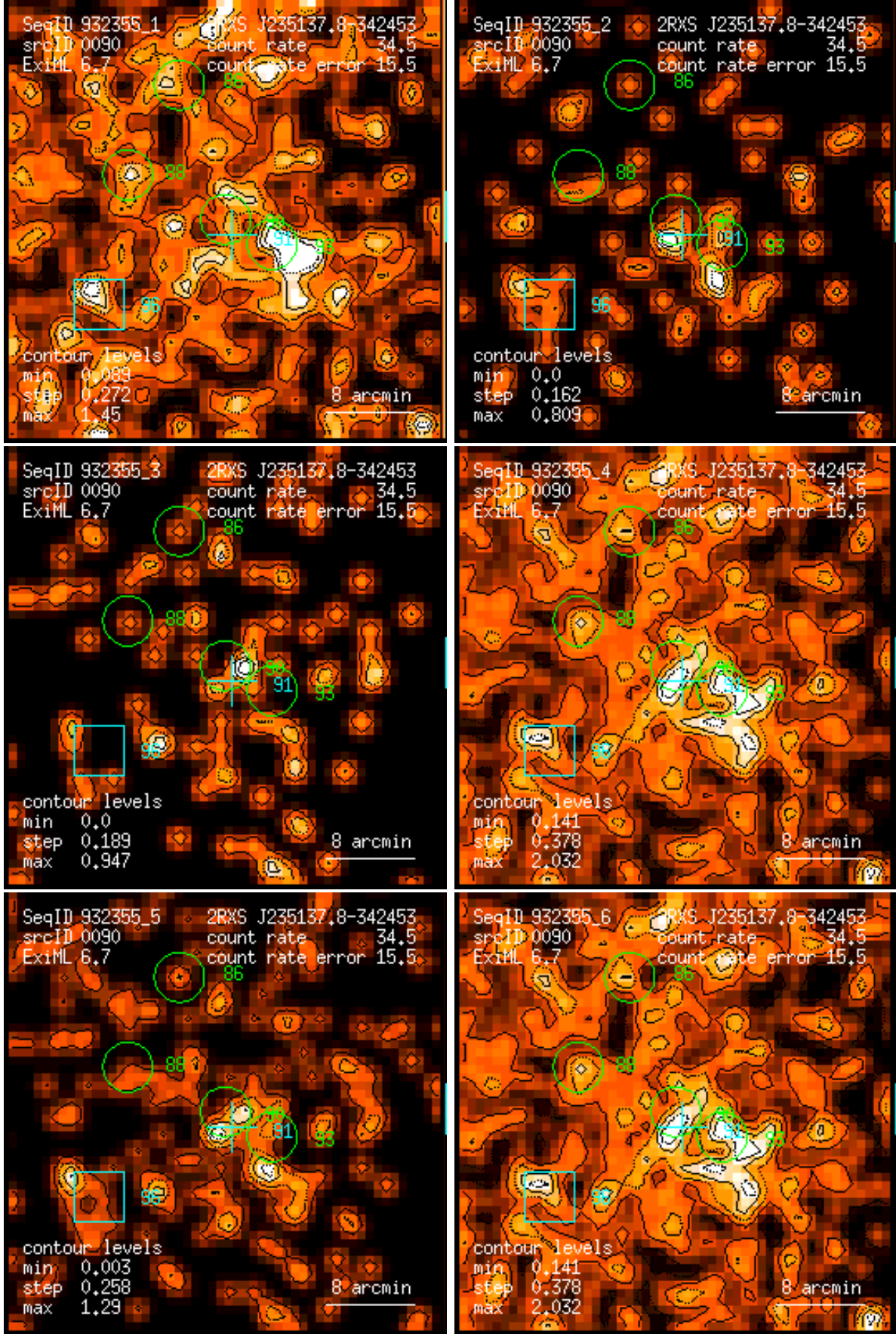
Figure 90: RASS 932355: detection 0090: band rate images, Gaussian filter: (1) PSPC channels 11 – 41, (2) 52 – 90, (3) 91 – 201, (4) 11 – 235, (5) 52 – 201, (6) 11 – 201. Broad band rates in counts/ks. Band rate contour levels in counts/ks/arcmin 2 .
