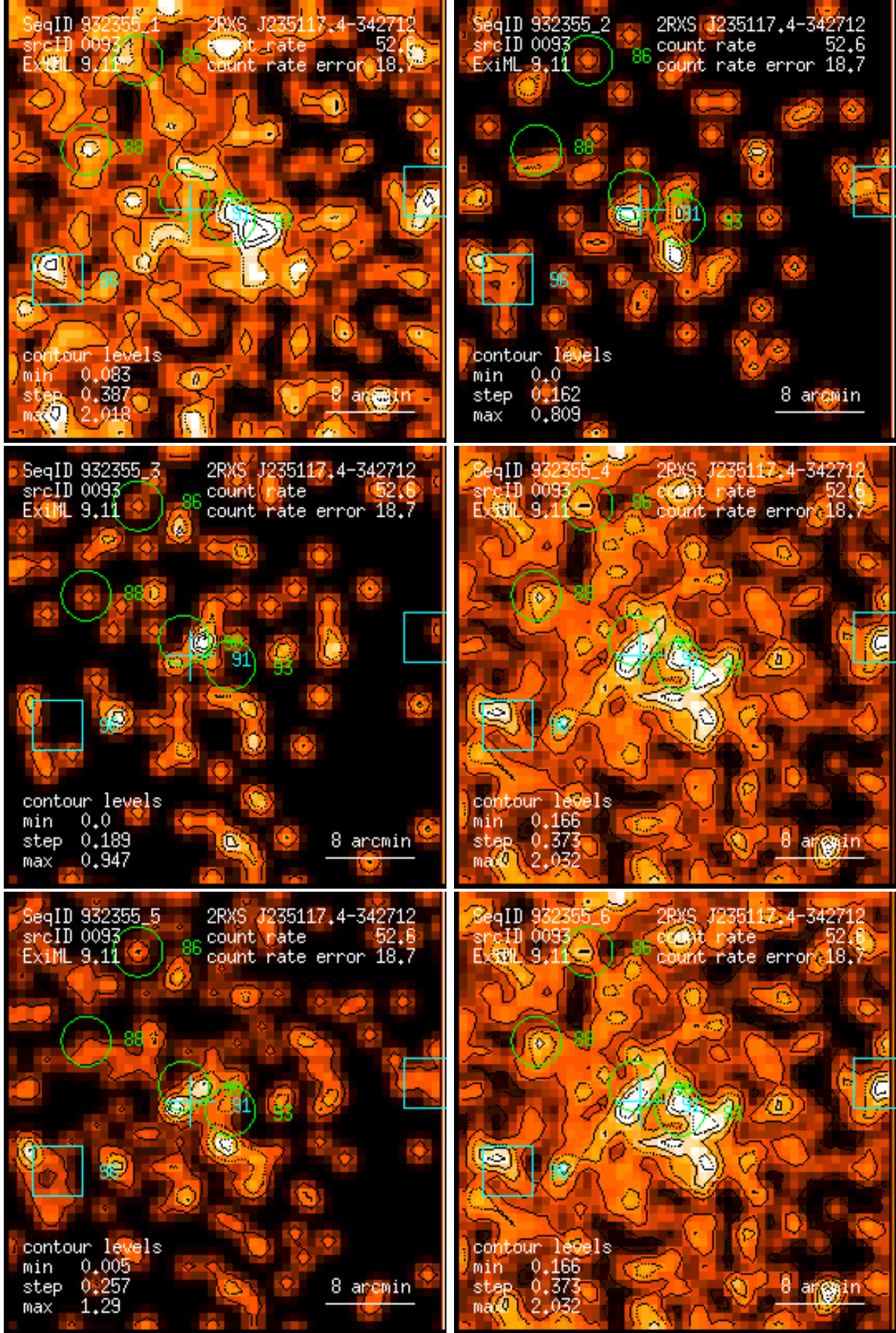
Figure 93: RASS 932355: detection 0093: band rate images, Gaussian filter: (1) PSPC channels 11 – 41, (2) 52 – 90, (3) 91 – 201, (4) 11 – 235, (5) 52 – 201, (6) 11 – 201. Broad band rates in counts/ks. Band rate contour levels in counts/ks/arcmin 2 .
