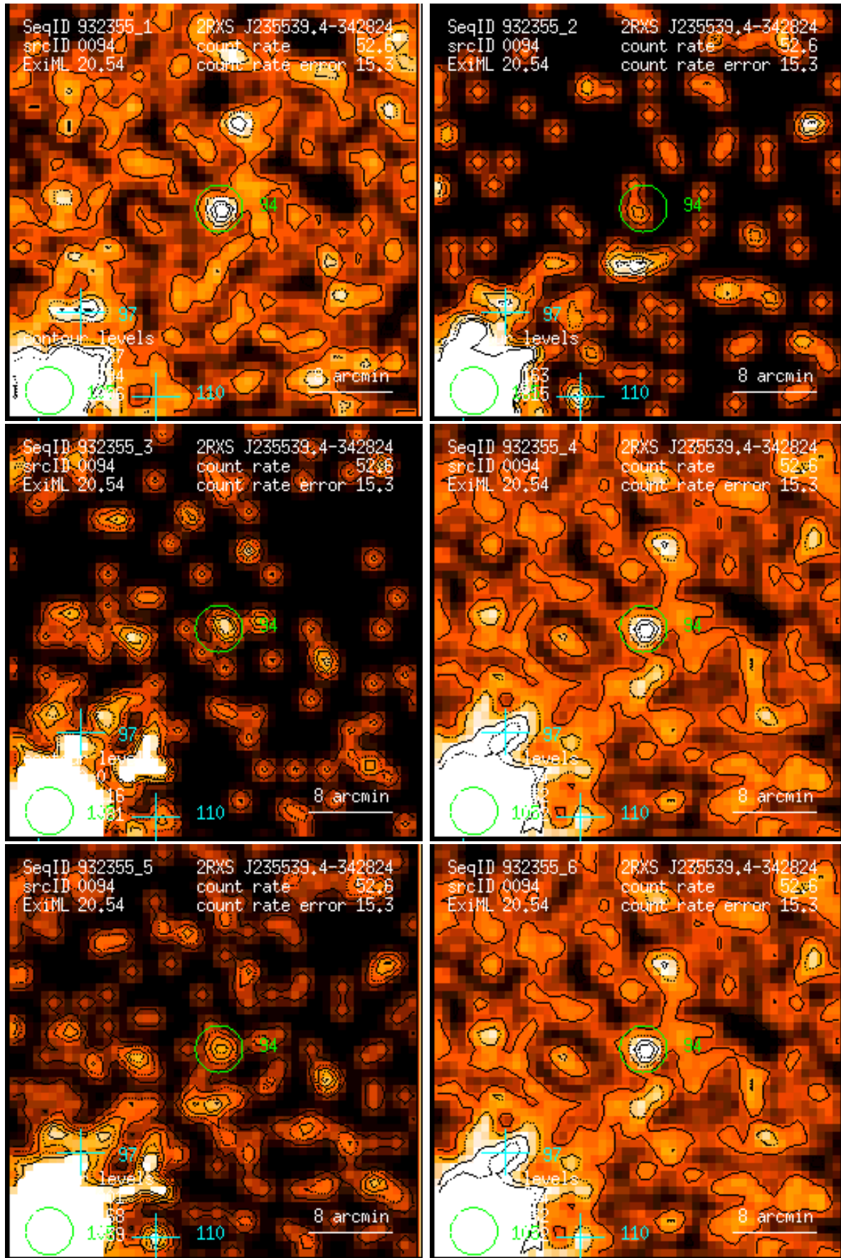
Figure 94: RASS 932355: detection 0094: band rate images, Gaussian filter: (1) PSPC channels 11 – 41, (2) 52 – 90, (3) 91 – 201, (4) 11 – 235, (5) 52 – 201, (6) 11 – 201. Broad band rates in counts/ks. Band rate contour levels in counts/ks/arcmin 2 .
