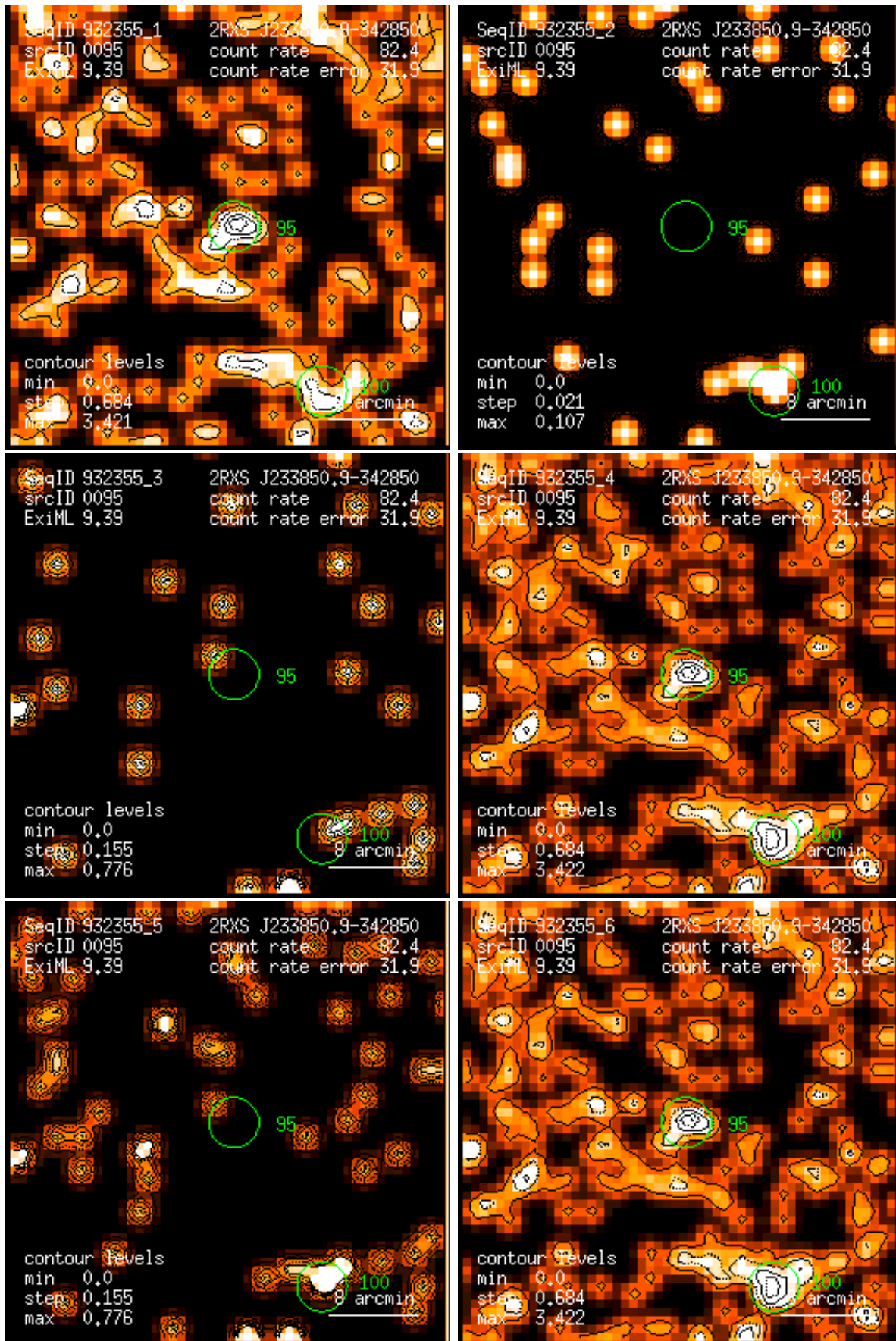
Figure 95: RASS 932355: detection 0095: band rate images, Gaussian filter: (1) PSPC channels 11 – 41, (2) 52 – 90, (3) 91 – 201, (4) 11 – 235, (5) 52 – 201, (6) 11 – 201. Broad band rates in counts/ks. Band rate contour levels in counts/ks/arcmin 2 .
