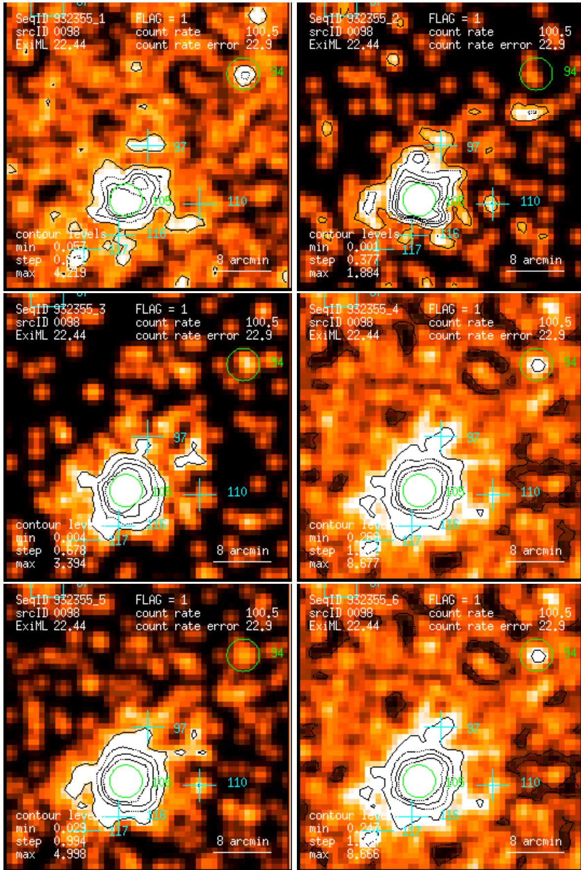
Figure 98: RASS 932355: detection 0098: band rate images, Gaussian filter: (1) PSPC channels 11 – 41, (2) 52 – 90, (3) 91 – 201, (4) 11 – 235, (5) 52 – 201, (6) 11 – 201. Broad band rates in counts/ks. Band rate contour levels in counts/ks/arcmin 2 .
