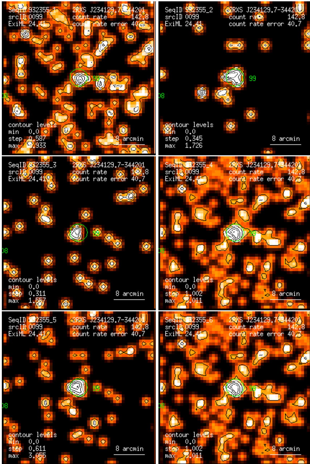
Figure 99: RASS 932355: detection 0099: band rate images, Gaussian filter: (1) PSPC channels 11 – 41, (2) 52 – 90, (3) 91 – 201, (4) 11 – 235, (5) 52 – 201, (6) 11 – 201. Broad band rates in counts/ks. Band rate contour levels in counts/ks/arcmin 2 .
