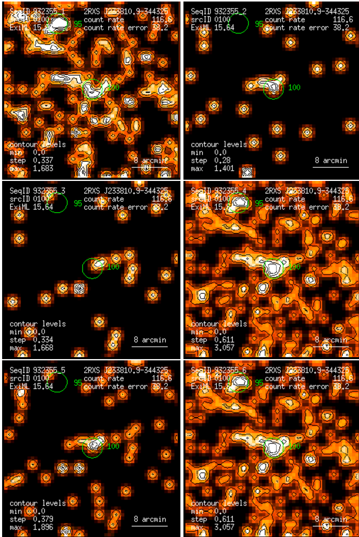
Figure 100: RASS 932355: detection 0100: band rate images, Gaussian filter: (1) PSPC channels 11 – 41, (2) 52 – 90, (3) 91 – 201, (4) 11 – 235, (5) 52 – 201, (6) 11 – 201. Broad band rates in counts/ks. Band rate contour levels in counts/ks/arcmin 2 .
