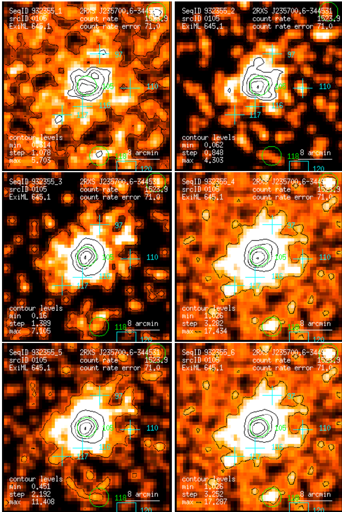
Figure 105: RASS 932355: detection 0105: band rate images, Gaussian filter: (1) PSPC channels 11 – 41, (2) 52 – 90, (3) 91 – 201, (4) 11 – 235, (5) 52 – 201, (6) 11 – 201. Broad band rates in counts/ks. Band rate contour levels in counts/ks/arcmin 2 .
