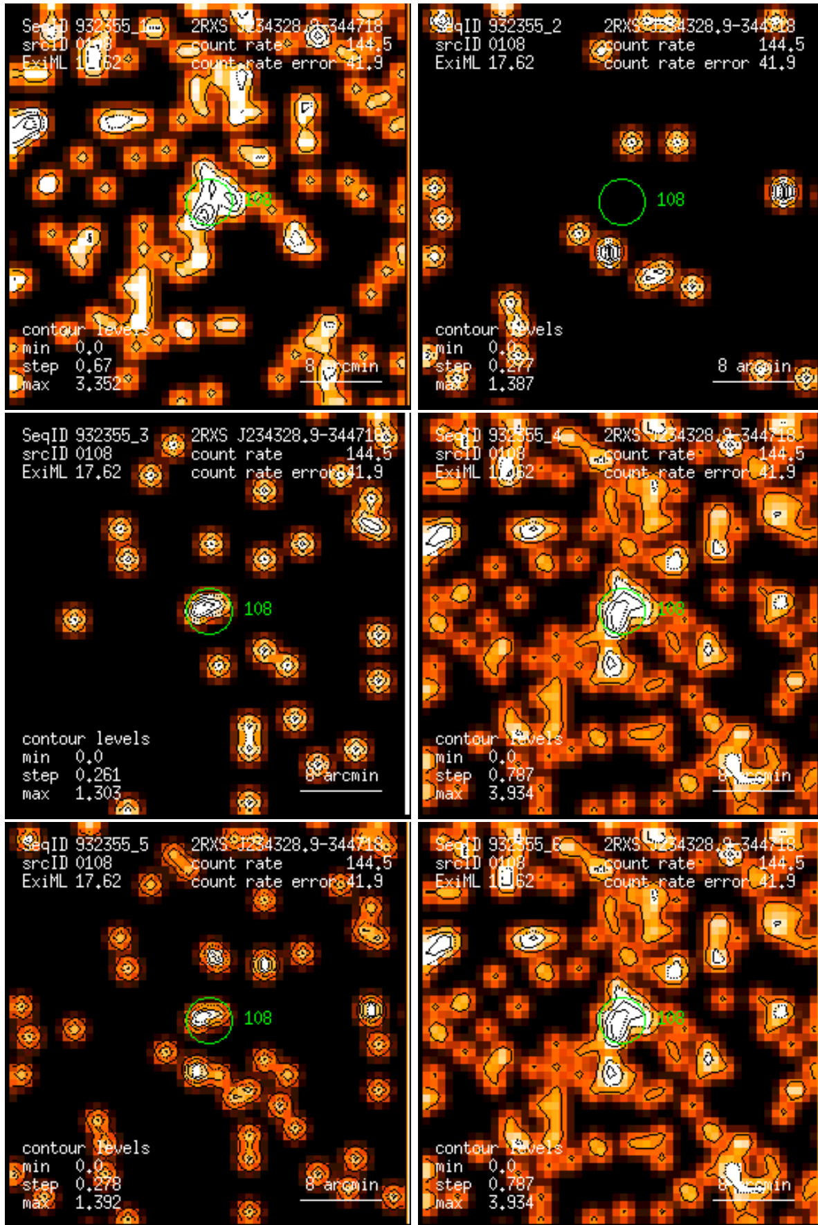
Figure 108: RASS 932355: detection 0108: band rate images, Gaussian filter: (1) PSPC channels 11 – 41, (2) 52 – 90, (3) 91 – 201, (4) 11 – 235, (5) 52 – 201, (6) 11 – 201. Broad band rates in counts/ks. Band rate contour levels in counts/ks/arcmin 2 .
