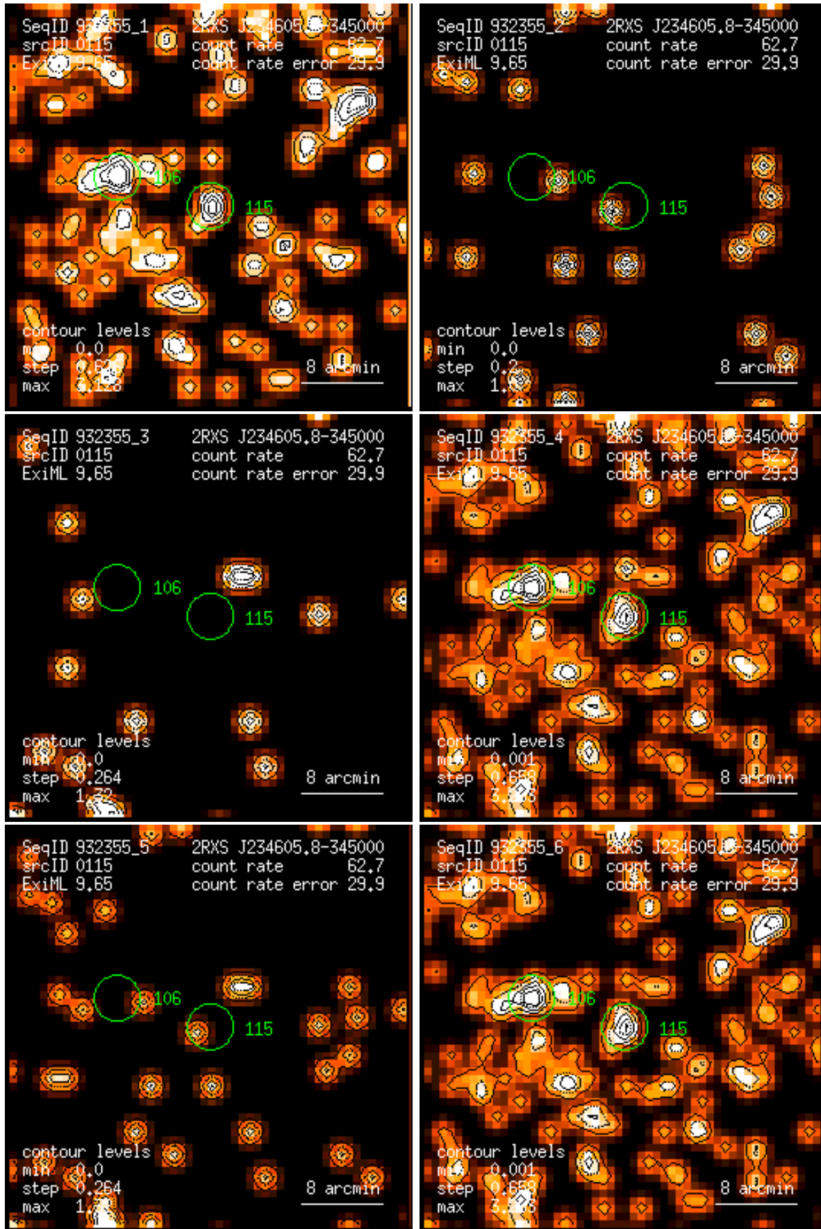
Figure 115: RASS 932355: detection 0115: band rate images, Gaussian filter: (1) PSPC channels 11 – 41, (2) 52 – 90, (3) 91 – 201, (4) 11 – 235, (5) 52 – 201, (6) 11 – 201. Broad band rates in counts/ks. Band rate contour levels in counts/ks/arcmin 2 .
