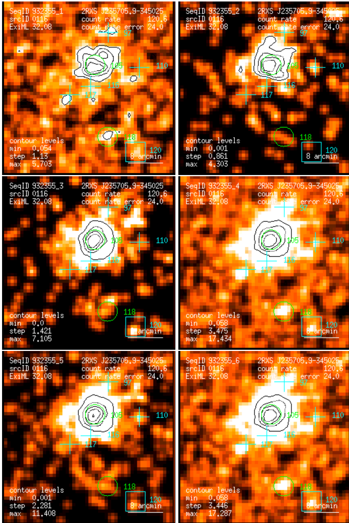
Figure 116: RASS 932355: detection 0116: band rate images, Gaussian filter: (1) PSPC channels 11 – 41, (2) 52 – 90, (3) 91 – 201, (4) 11 – 235, (5) 52 – 201, (6) 11 – 201. Broad band rates in counts/ks. Band rate contour levels in counts/ks/arcmin 2 .
