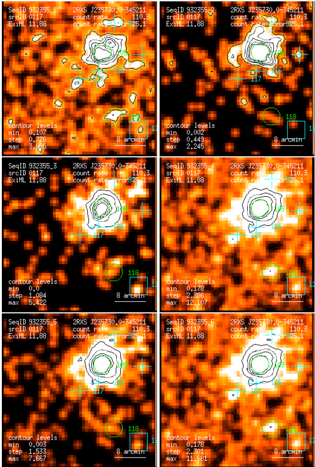
Figure 117: RASS 932355: detection 0117: band rate images, Gaussian filter: (1) PSPC channels 11 – 41, (2) 52 – 90, (3) 91 – 201, (4) 11 – 235, (5) 52 – 201, (6) 11 – 201. Broad band rates in counts/ks. Band rate contour levels in counts/ks/arcmin 2 .
