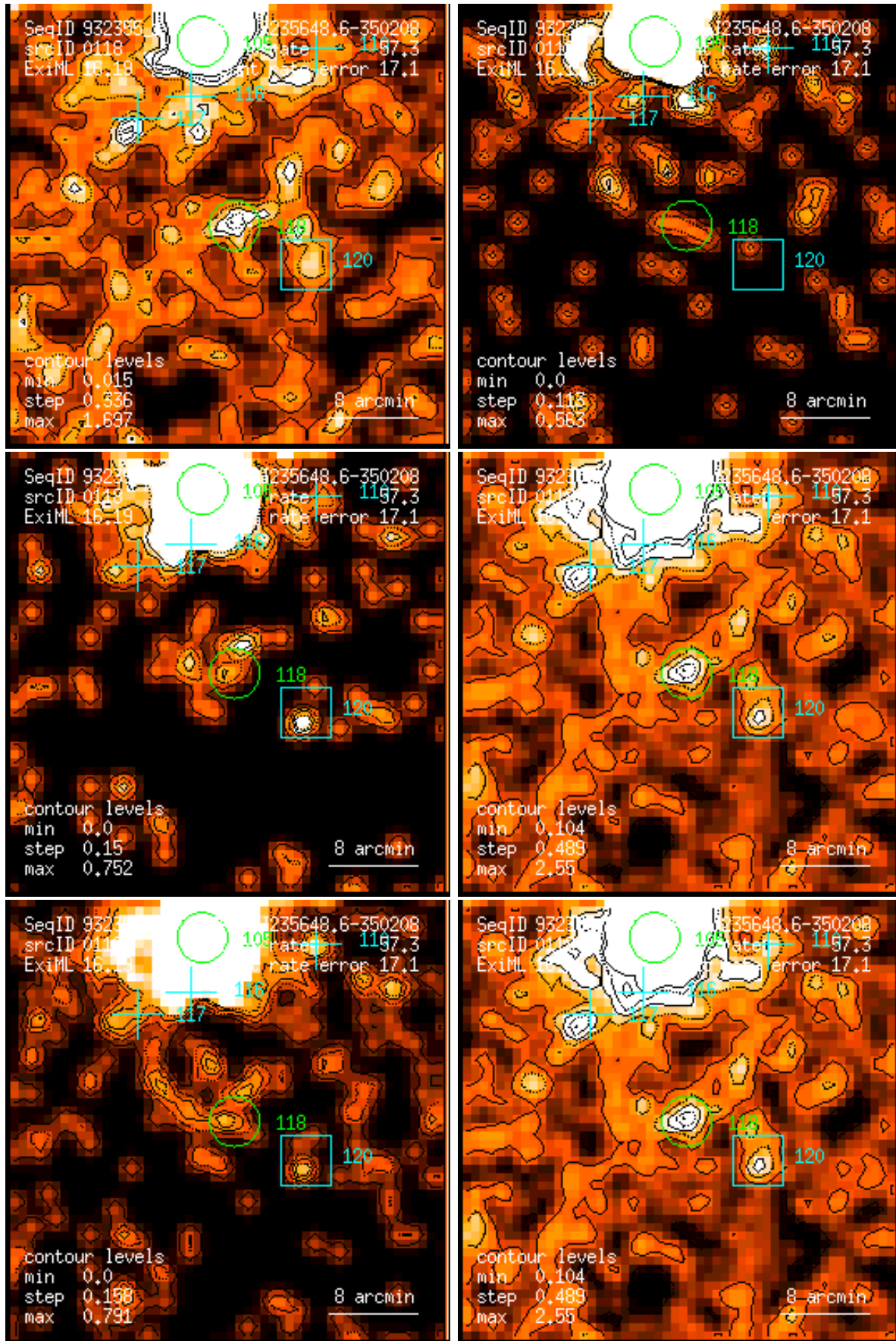
Figure 118: RASS 932355: detection 0118: band rate images, Gaussian filter: (1) PSPC channels 11 – 41, (2) 52 – 90, (3) 91 – 201, (4) 11 – 235, (5) 52 – 201, (6) 11 – 201. Broad band rates in counts/ks. Band rate contour levels in counts/ks/arcmin 2 .
