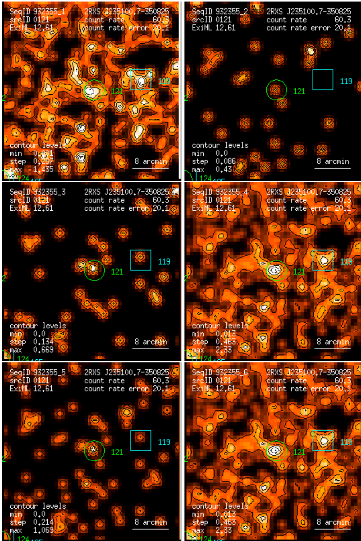
Figure 121: RASS 932355: detection 0121: band rate images, Gaussian filter: (1) PSPC channels 11 – 41, (2) 52 – 90, (3) 91 – 201, (4) 11 – 235, (5) 52 – 201, (6) 11 – 201. Broad band rates in counts/ks. Band rate contour levels in counts/ks/arcmin 2 .
