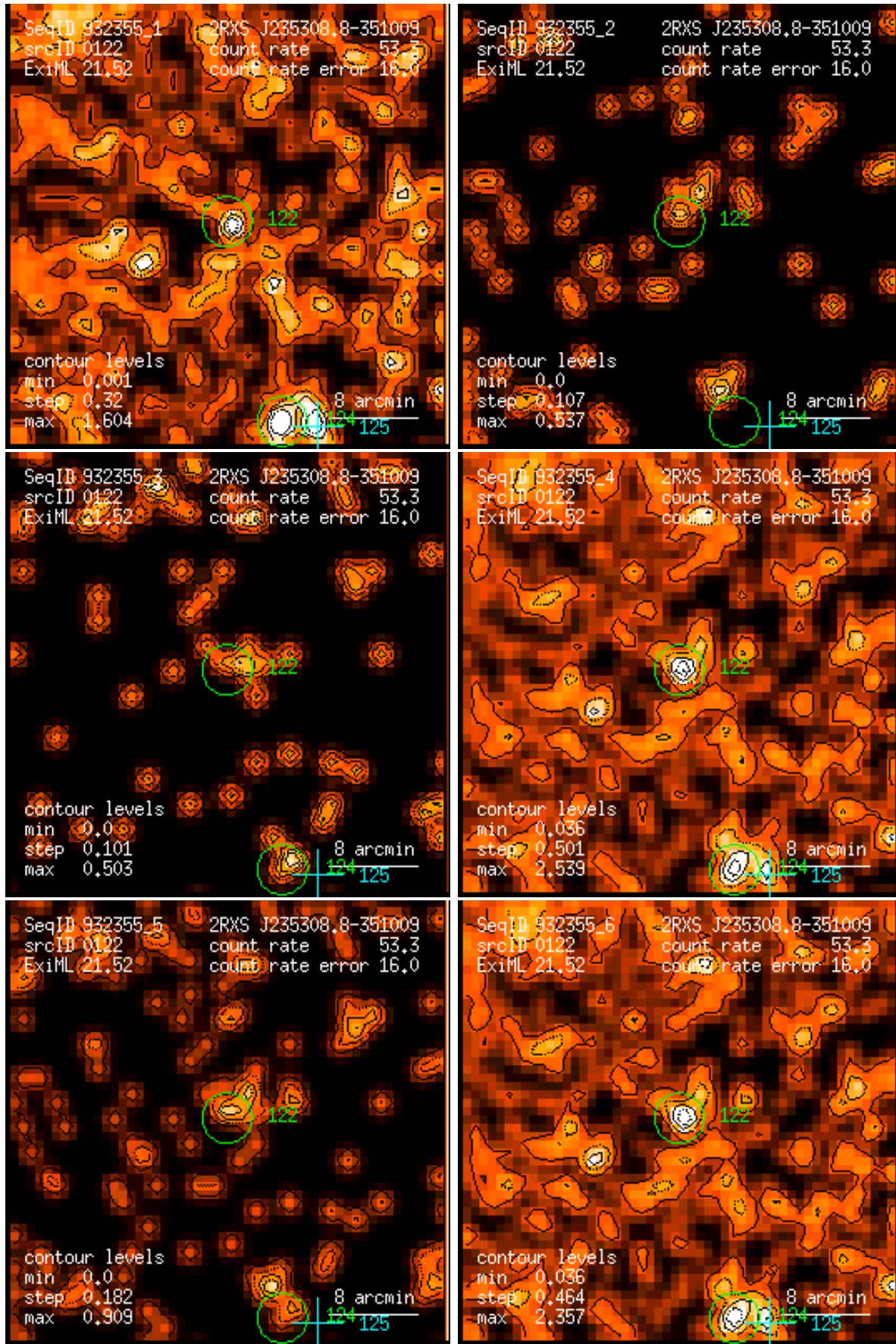
Figure 122: RASS 932355: detection 0122: band rate images, Gaussian filter: (1) PSPC channels 11 – 41, (2) 52 – 90, (3) 91 – 201, (4) 11 – 235, (5) 52 – 201, (6) 11 – 201. Broad band rates in counts/ks. Band rate contour levels in counts/ks/arcmin 2 .
