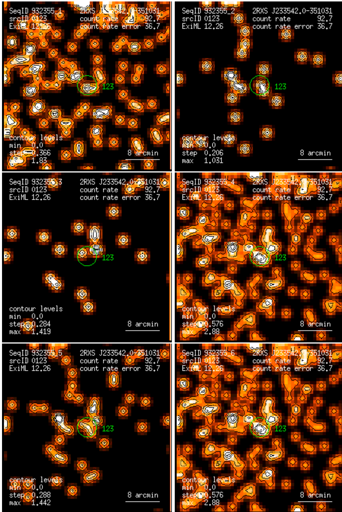
Figure 123: RASS 932355: detection 0123: band rate images, Gaussian filter: (1) PSPC channels 11 – 41, (2) 52 – 90, (3) 91 – 201, (4) 11 – 235, (5) 52 – 201, (6) 11 – 201. Broad band rates in counts/ks. Band rate contour levels in counts/ks/arcmin 2 .
