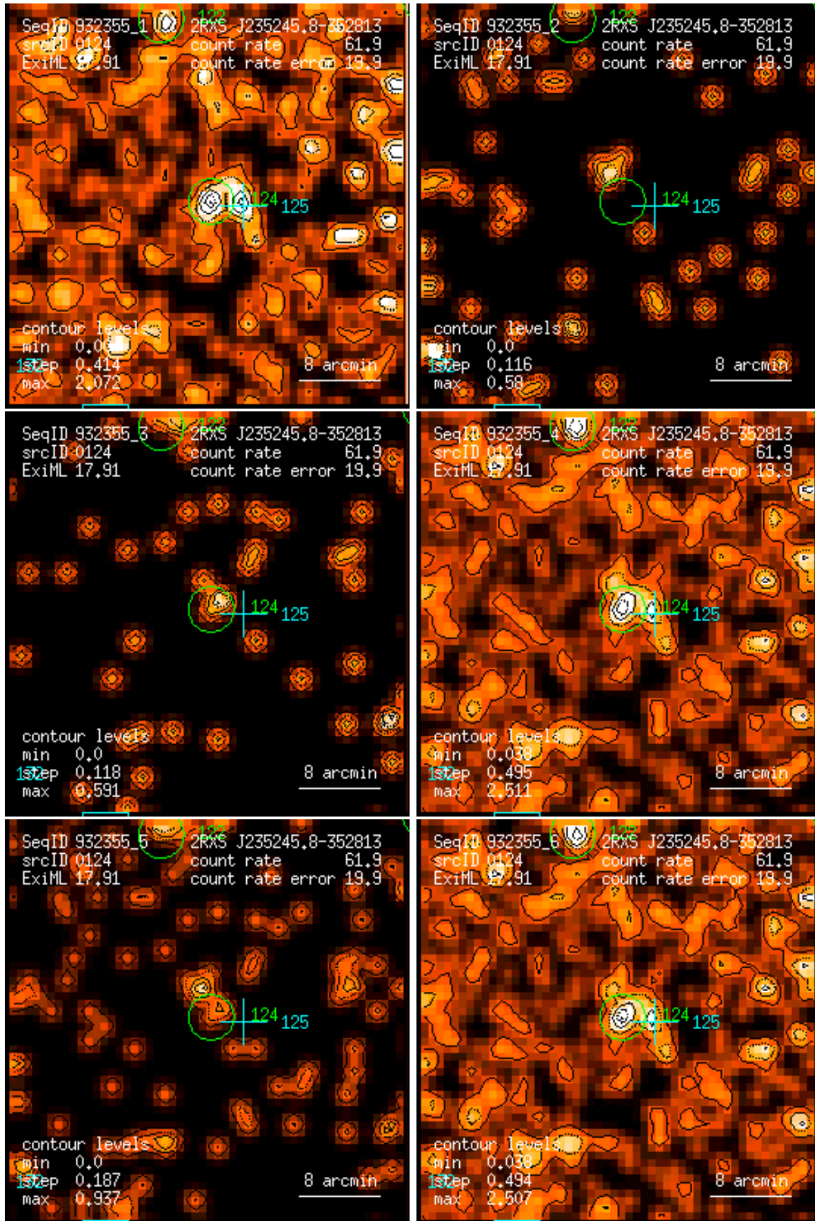
Figure 124: RASS 932355: detection 0124: band rate images, Gaussian filter: (1) PSPC channels 11 – 41, (2) 52 – 90, (3) 91 – 201, (4) 11 – 235, (5) 52 – 201, (6) 11 – 201. Broad band rates in counts/ks. Band rate contour levels in counts/ks/arcmin 2 .
