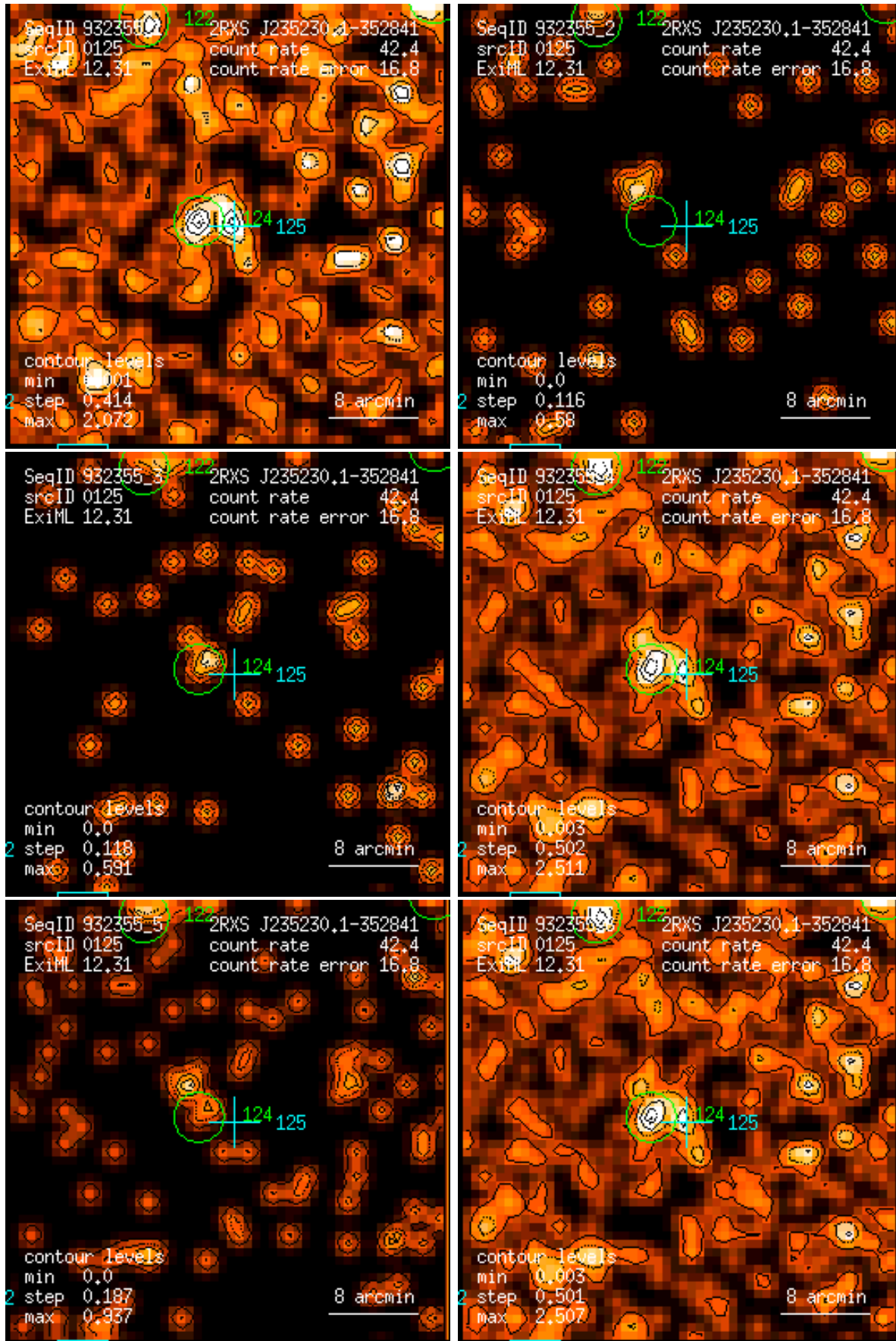
Figure 125: RASS 932355: detection 0125: band rate images, Gaussian filter: (1) PSPC channels 11 – 41, (2) 52 – 90, (3) 91 – 201, (4) 11 – 235, (5) 52 – 201, (6) 11 – 201. Broad band rates in counts/ks. Band rate contour levels in counts/ks/arcmin 2 .
