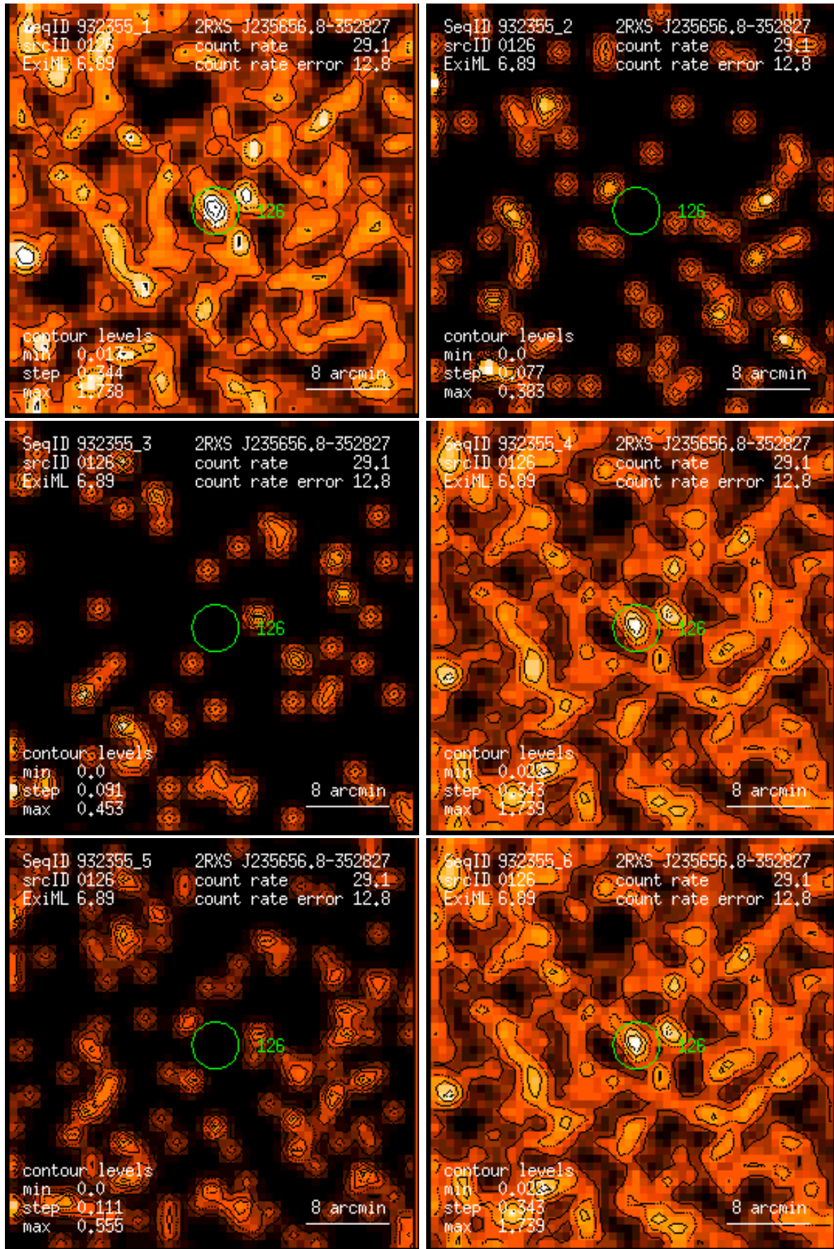
Figure 126: RASS 932355: detection 0126: band rate images, Gaussian filter: (1) PSPC channels 11 – 41, (2) 52 – 90, (3) 91 – 201, (4) 11 – 235, (5) 52 – 201, (6) 11 – 201. Broad band rates in counts/ks. Band rate contour levels in counts/ks/arcmin 2 .
