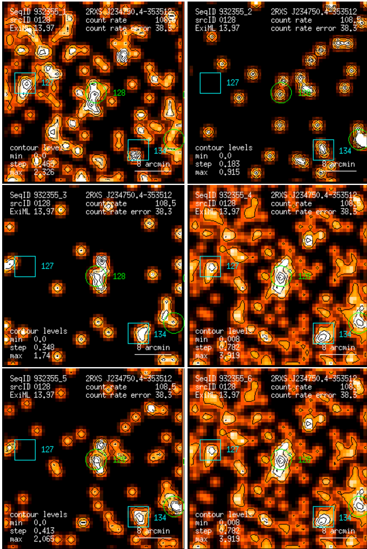
Figure 128: RASS 932355: detection 0128: band rate images, Gaussian filter: (1) PSPC channels 11 – 41, (2) 52 – 90, (3) 91 – 201, (4) 11 – 235, (5) 52 – 201, (6) 11 – 201. Broad band rates in counts/ks. Band rate contour levels in counts/ks/arcmin 2 .
