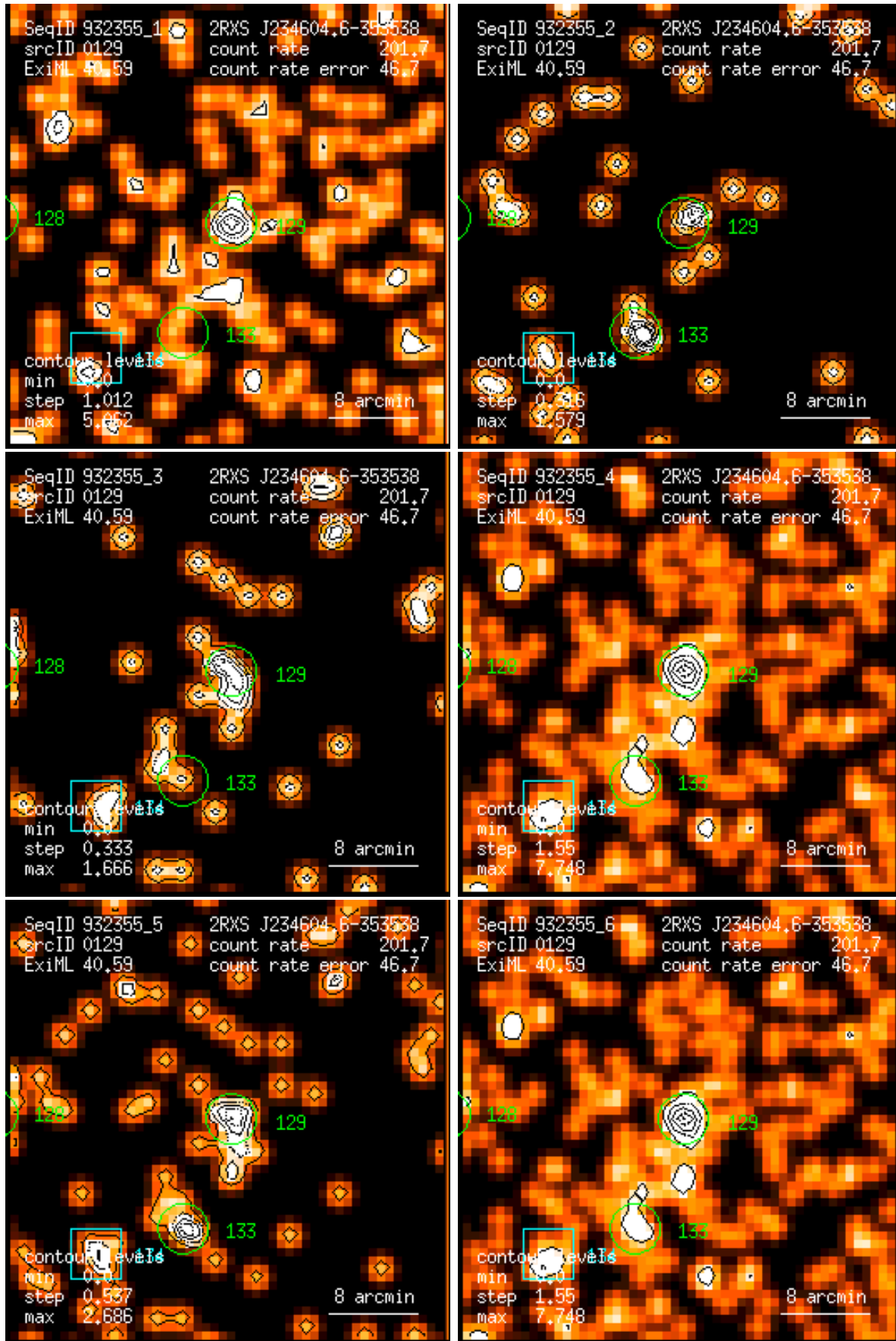
Figure 129: RASS 932355: detection 0129: band rate images, Gaussian filter: (1) PSPC channels 11 – 41, (2) 52 – 90, (3) 91 – 201, (4) 11 – 235, (5) 52 – 201, (6) 11 – 201. Broad band rates in counts/ks. Band rate contour levels in counts/ks/arcmin 2 .
