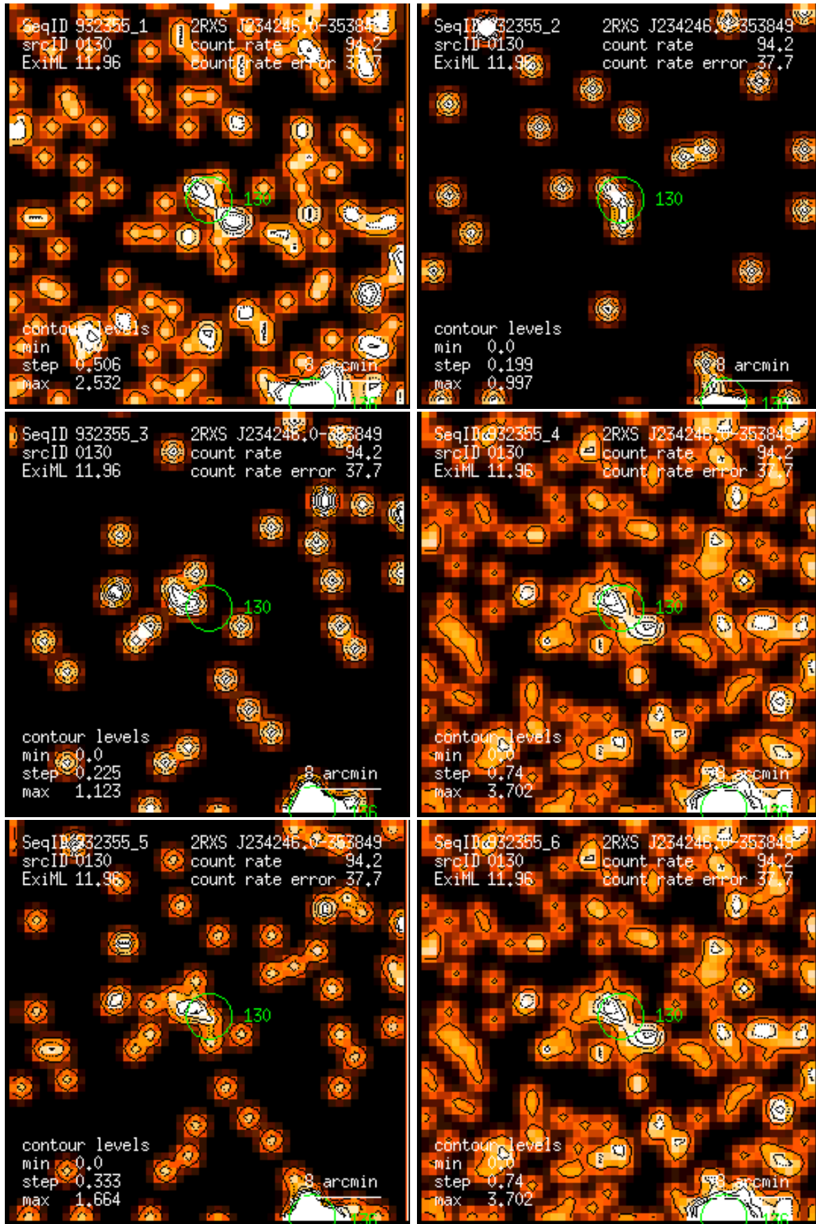
Figure 130: RASS 932355: detection 0130: band rate images, Gaussian filter: (1) PSPC channels 11 – 41, (2) 52 – 90, (3) 91 – 201, (4) 11 – 235, (5) 52 – 201, (6) 11 – 201. Broad band rates in counts/ks. Band rate contour levels in counts/ks/arcmin 2 .
