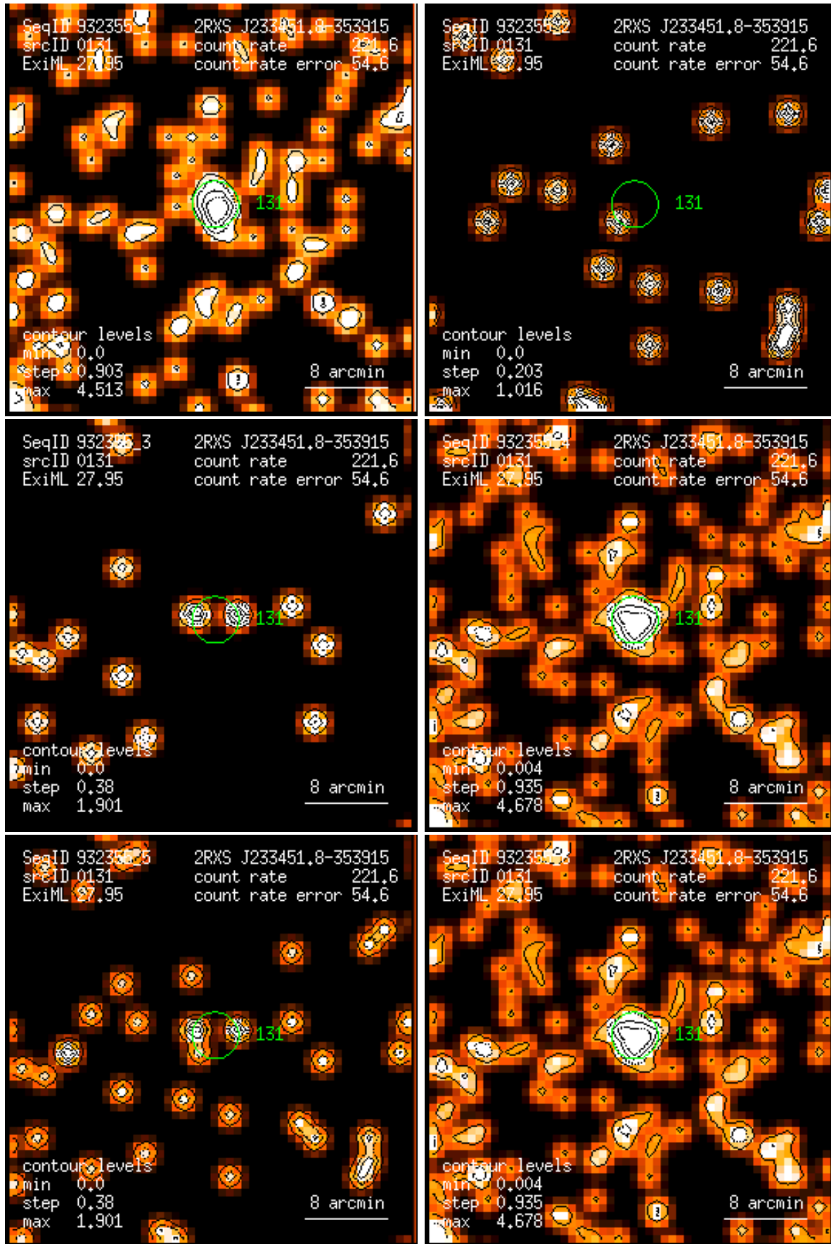
Figure 131: RASS 932355: detection 0131: band rate images, Gaussian filter: (1) PSPC channels 11 – 41, (2) 52 – 90, (3) 91 – 201, (4) 11 – 235, (5) 52 – 201, (6) 11 – 201. Broad band rates in counts/ks. Band rate contour levels in counts/ks/arcmin 2 .
