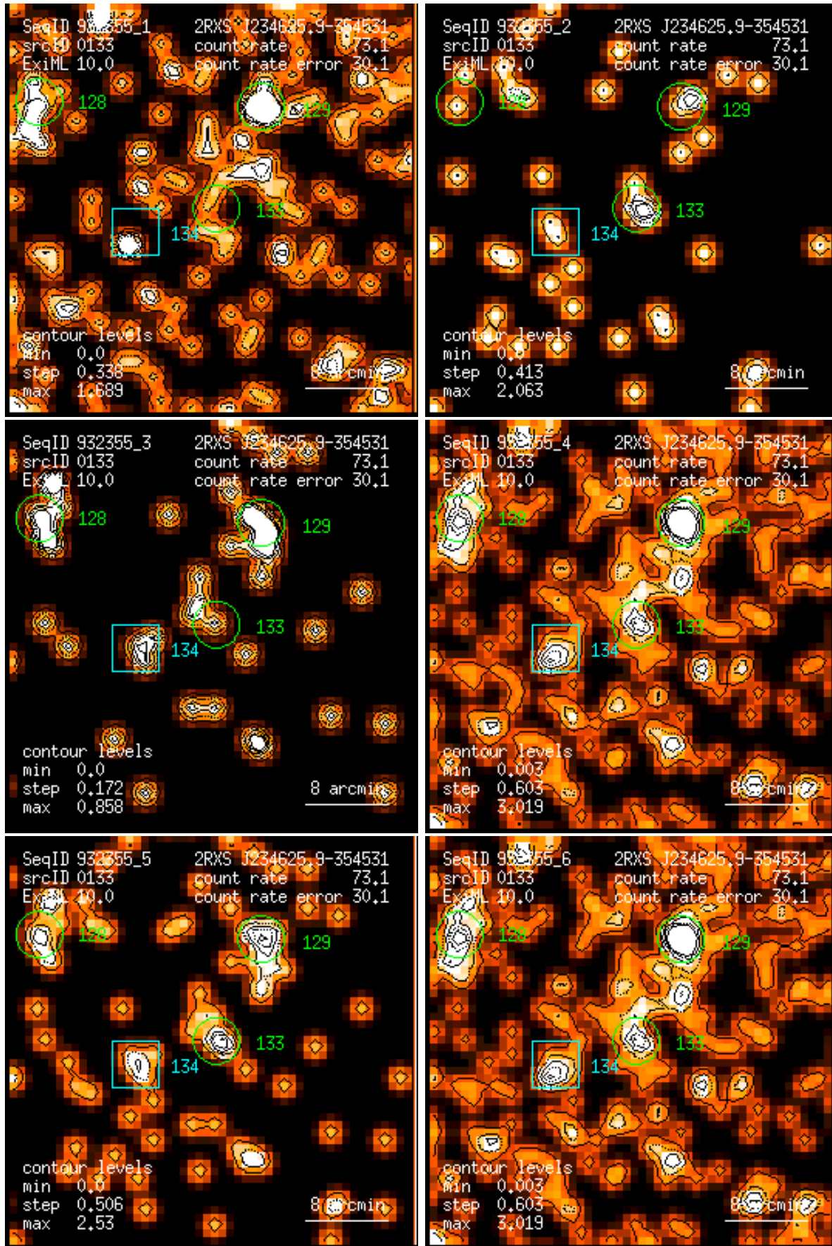
Figure 133: RASS 932355: detection 0133: band rate images, Gaussian filter: (1) PSPC channels 11 – 41, (2) 52 – 90, (3) 91 – 201, (4) 11 – 235, (5) 52 – 201, (6) 11 – 201. Broad band rates in counts/ks. Band rate contour levels in counts/ks/arcmin 2 .
