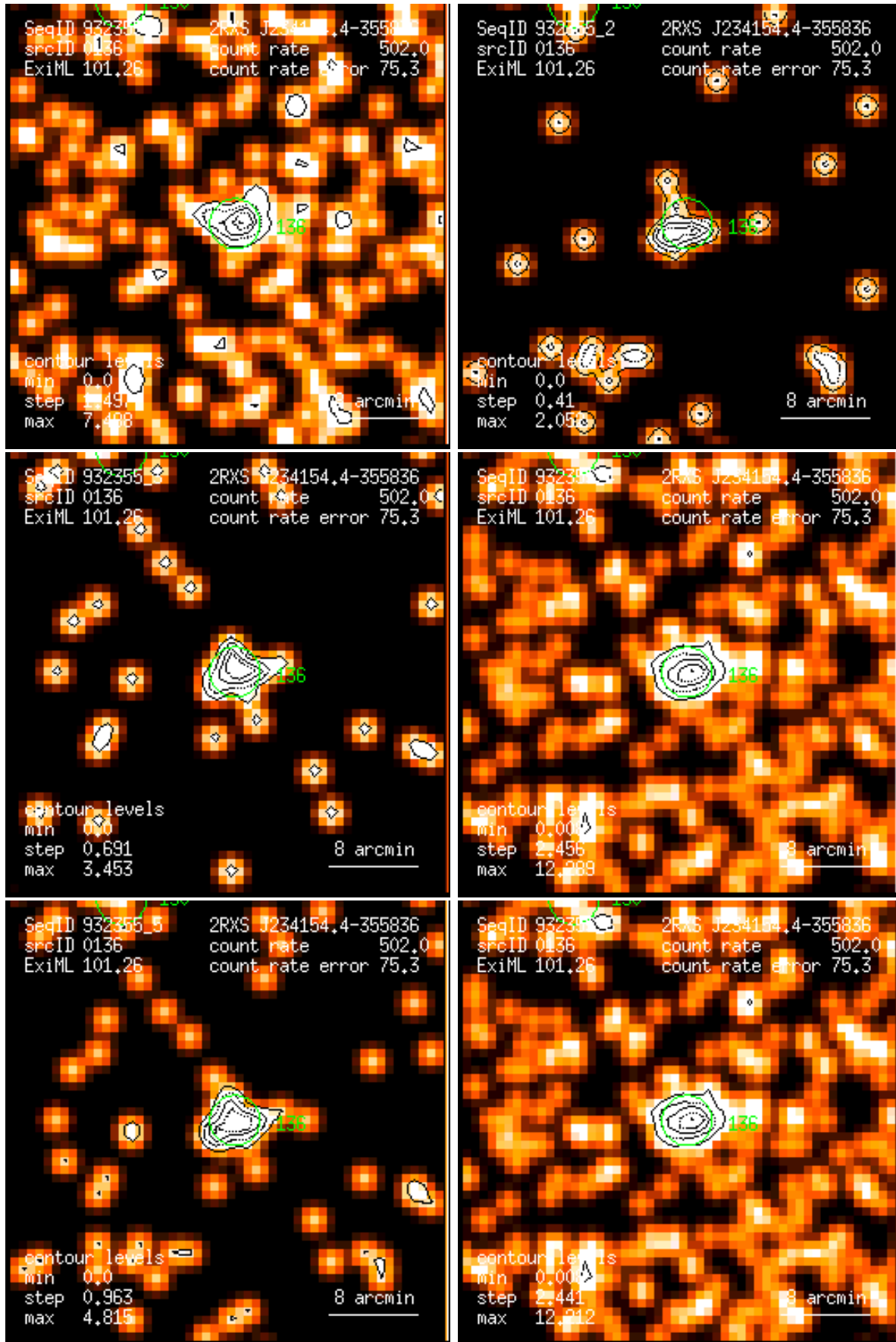
Figure 136: RASS 932355: detection 0136: band rate images, Gaussian filter: (1) PSPC channels 11 – 41, (2) 52 – 90, (3) 91 – 201, (4) 11 – 235, (5) 52 – 201, (6) 11 – 201. Broad band rates in counts/ks. Band rate contour levels in counts/ks/arcmin 2 .
