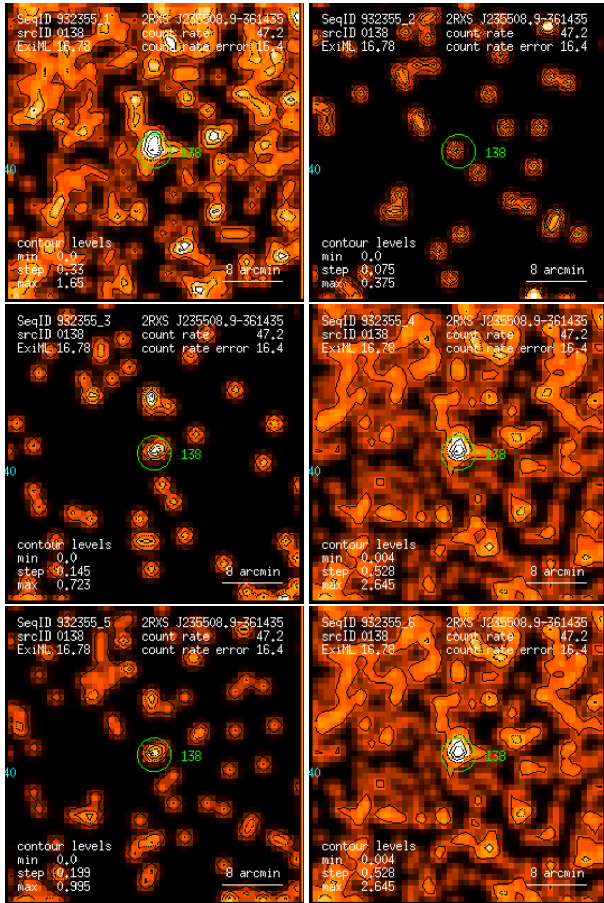
Figure 138: RASS 932355: detection 0138: band rate images, Gaussian filter: (1) PSPC channels 11 – 41, (2) 52 – 90, (3) 91 – 201, (4) 11 – 235, (5) 52 – 201, (6) 11 – 201. Broad band rates in counts/ks. Band rate contour levels in counts/ks/arcmin 2 .
