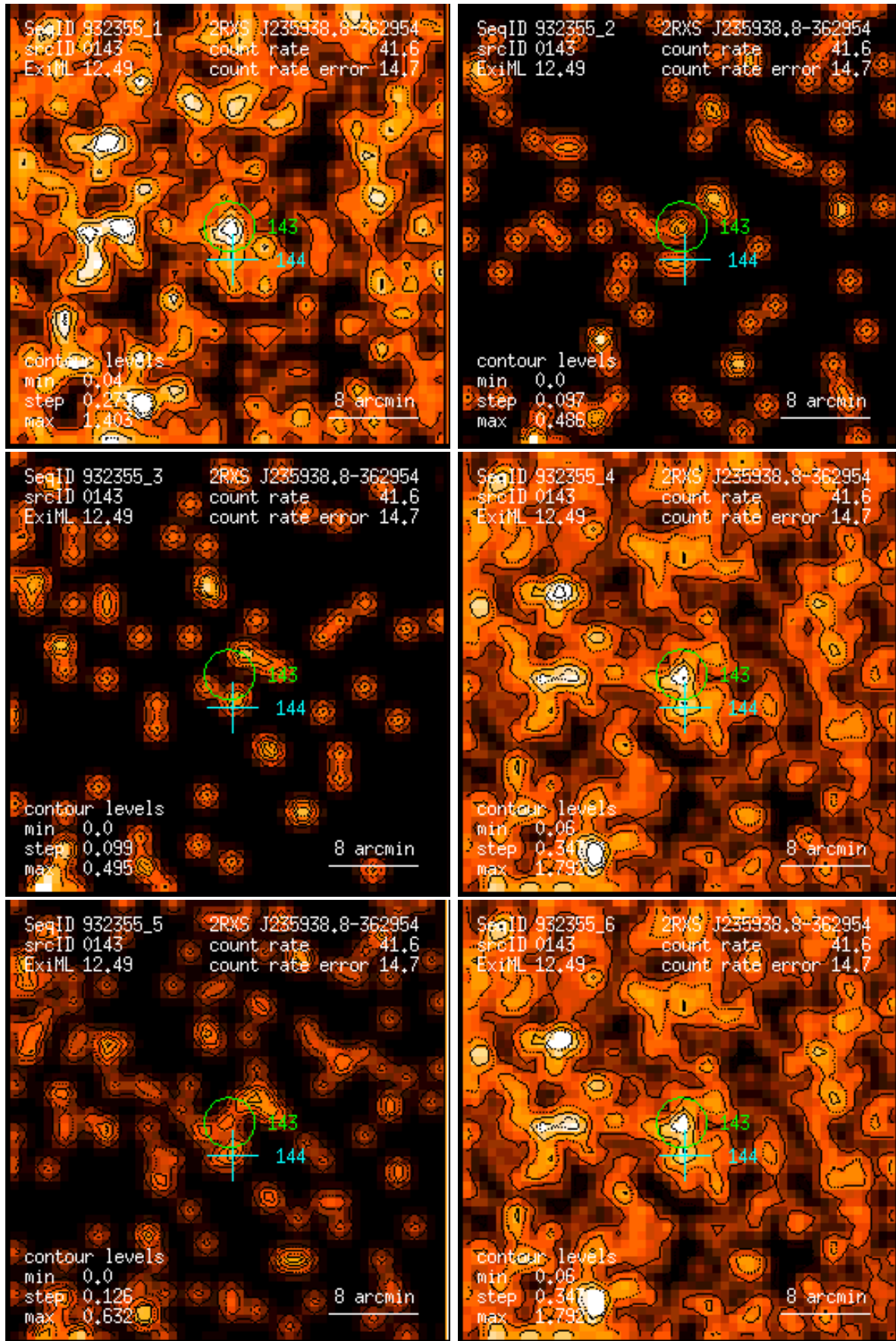
Figure 143: RASS 932355: detection 0143: band rate images, Gaussian filter: (1) PSPC channels 11 – 41, (2) 52 – 90, (3) 91 – 201, (4) 11 – 235, (5) 52 – 201, (6) 11 – 201. Broad band rates in counts/ks. Band rate contour levels in counts/ks/arcmin 2 .
