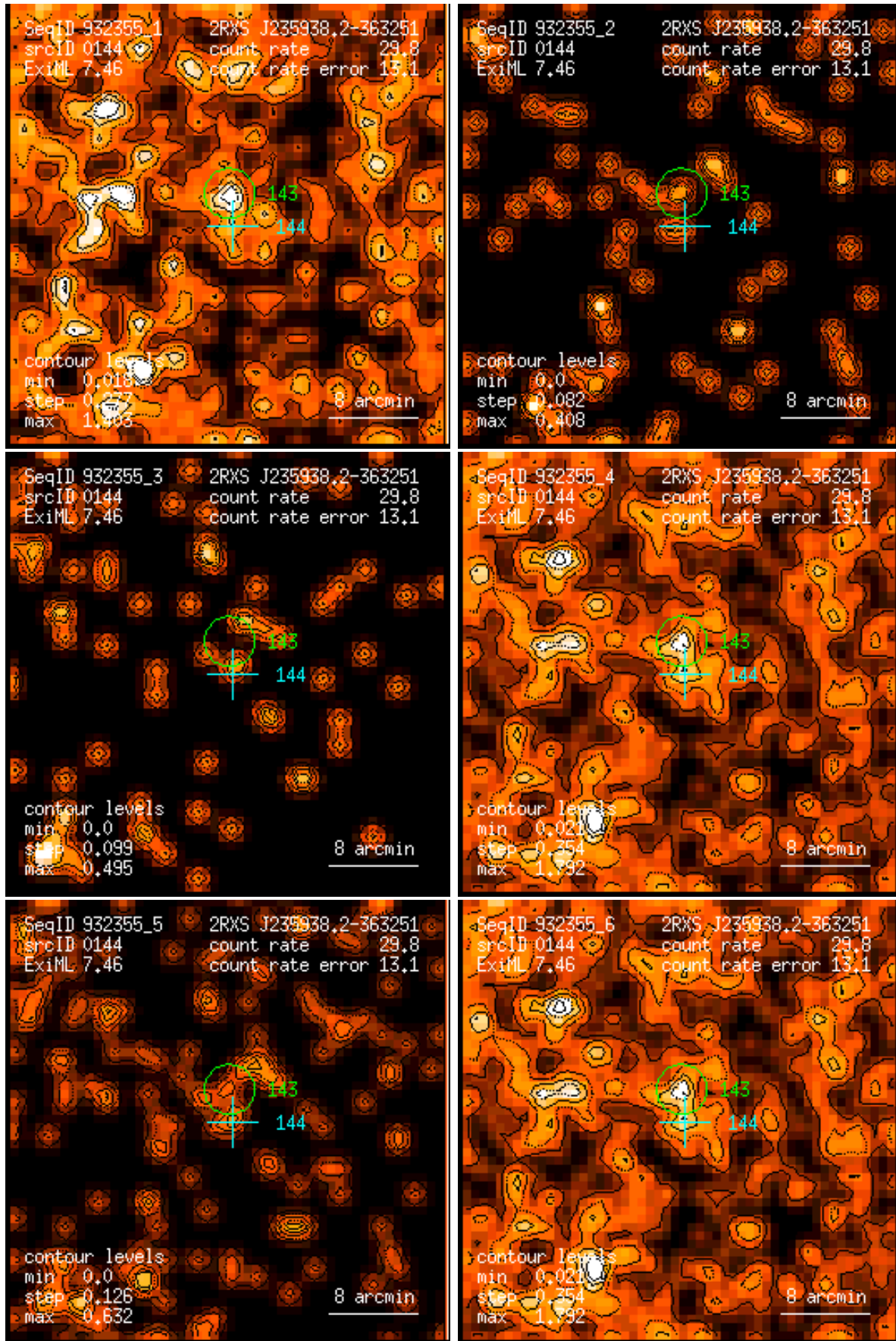
Figure 144: RASS 932355: detection 0144: band rate images, Gaussian filter: (1) PSPC channels 11 – 41, (2) 52 – 90, (3) 91 – 201, (4) 11 – 235, (5) 52 – 201, (6) 11 – 201. Broad band rates in counts/ks. Band rate contour levels in counts/ks/arcmin 2 .
