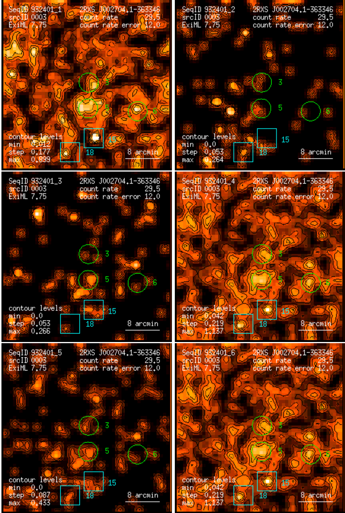
Figure 3: RASS 932401: detection 0003: band rate images, Gaussian filter: (1) PSPC channels 11 – 41, (2) 52 – 90, (3) 91 – 201, (4) 11 – 235, (5) 52 – 201, (6) 11 – 201. Broad band rates in counts/ks. Band rate contour levels in counts/ks/arcmin 2 .
