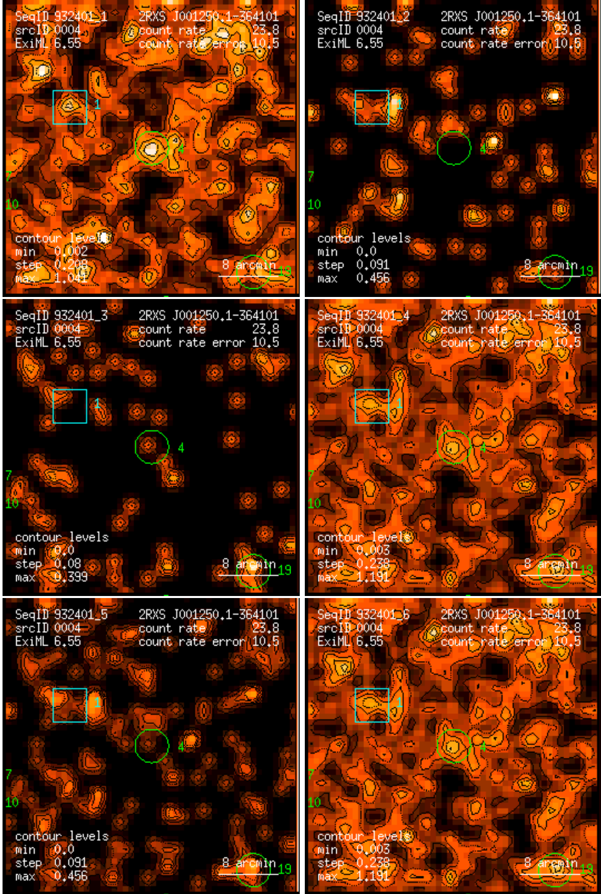
Figure 4: RASS 932401: detection 0004: band rate images, Gaussian filter: (1) PSPC channels 11 – 41, (2) 52 – 90, (3) 91 – 201, (4) 11 – 235, (5) 52 – 201, (6) 11 – 201. Broad band rates in counts/ks. Band rate contour levels in counts/ks/arcmin 2 .
