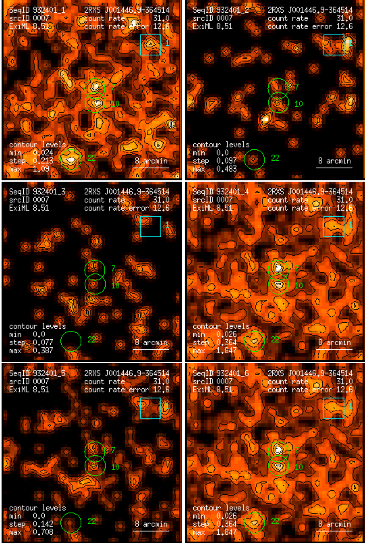
Figure 7: RASS 932401: detection 0007: band rate images, Gaussian filter: (1) PSPC channels 11 – 41, (2) 52 – 90, (3) 91 – 201, (4) 11 – 235, (5) 52 – 201, (6) 11 – 201. Broad band rates in counts/ks. Band rate contour levels in counts/ks/arcmin 2 .
