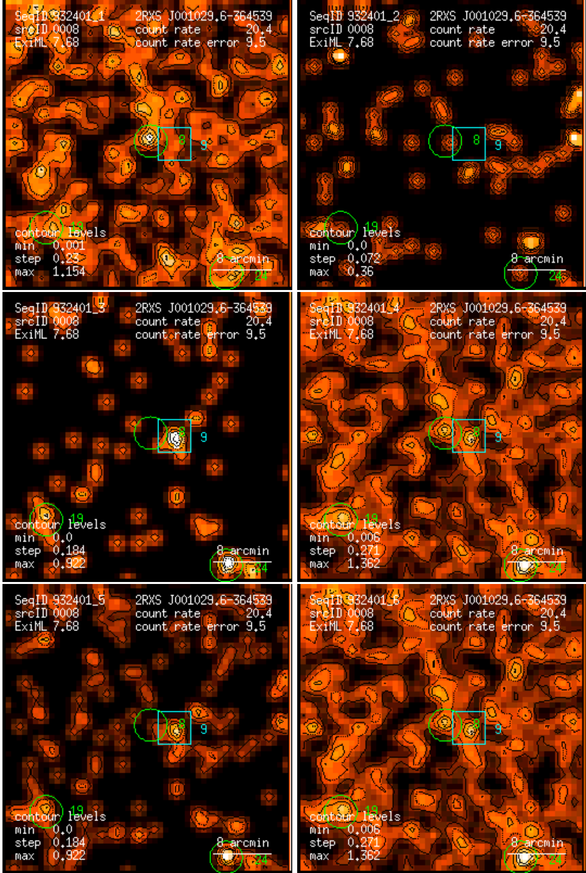
Figure 8: RASS 932401: detection 0008: band rate images, Gaussian filter: (1) PSPC channels 11 – 41, (2) 52 – 90, (3) 91 – 201, (4) 11 – 235, (5) 52 – 201, (6) 11 – 201. Broad band rates in counts/ks. Band rate contour levels in counts/ks/arcmin 2 .
