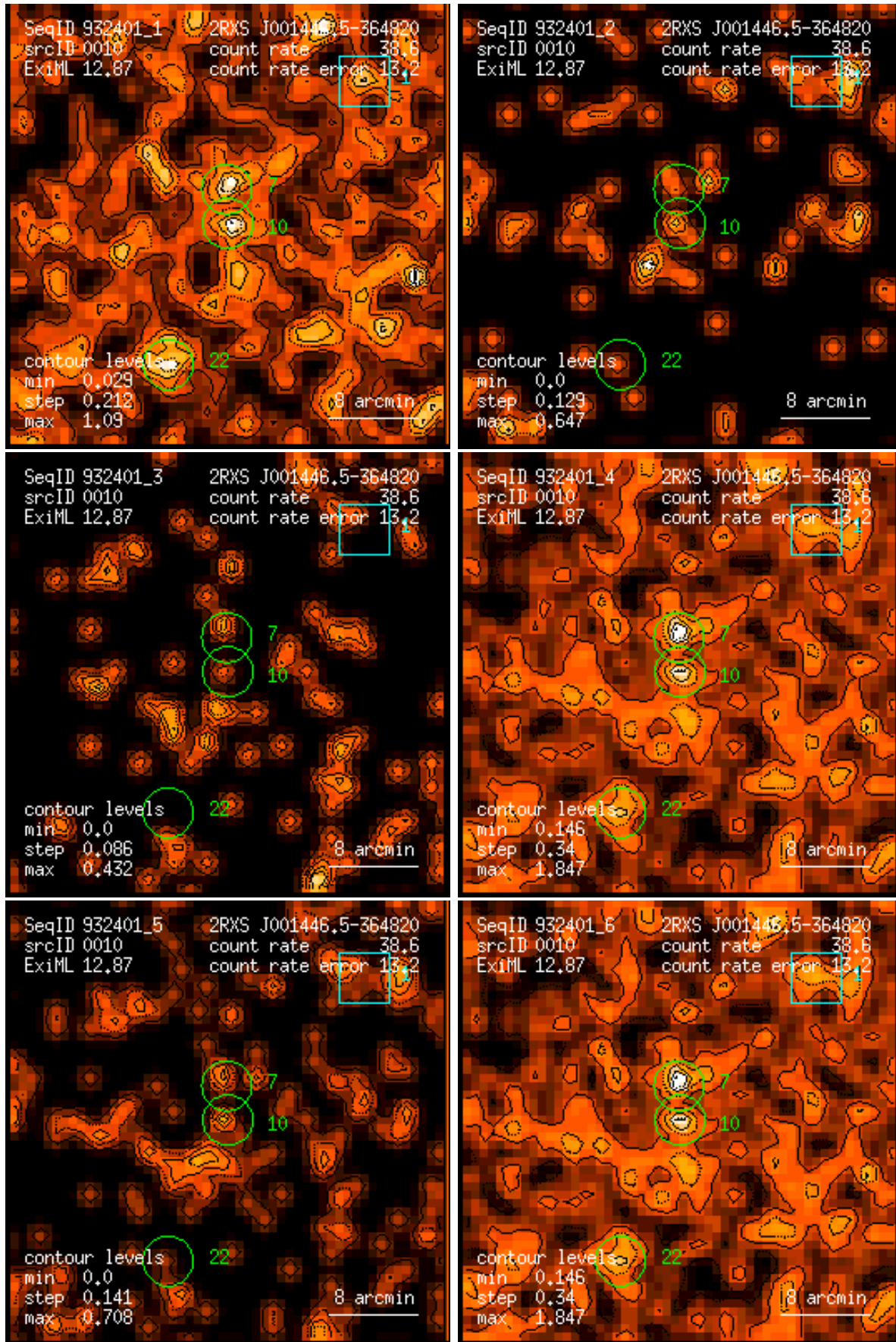
Figure 10: RASS 932401: detection 0010: band rate images, Gaussian filter: (1) PSPC channels 11 – 41, (2) 52 – 90, (3) 91 – 201, (4) 11 – 235, (5) 52 – 201, (6) 11 – 201. Broad band rates in counts/ks. Band rate contour levels in counts/ks/arcmin 2 .
