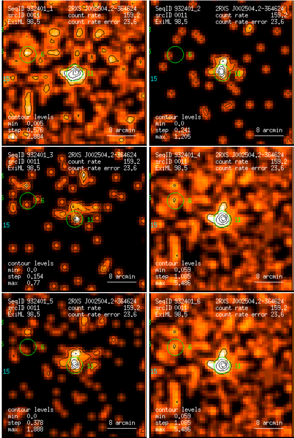
Figure 11: RASS 932401: detection 0011: band rate images, Gaussian filter: (1) PSPC channels 11 – 41, (2) 52 – 90, (3) 91 – 201, (4) 11 – 235, (5) 52 – 201, (6) 11 – 201. Broad band rates in counts/ks. Band rate contour levels in counts/ks/arcmin 2 .
