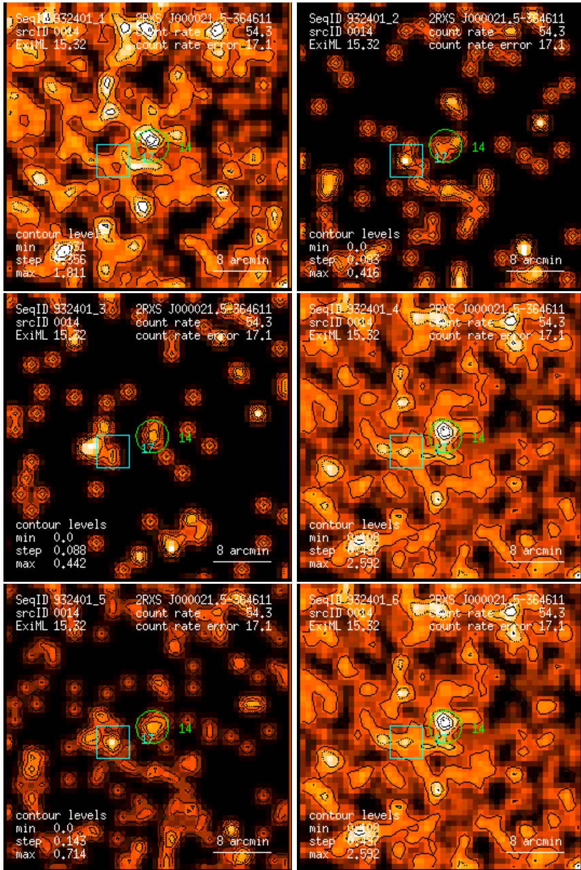
Figure 14: RASS 932401: detection 0014: band rate images, Gaussian filter: (1) PSPC channels 11 – 41, (2) 52 – 90, (3) 91 – 201, (4) 11 – 235, (5) 52 – 201, (6) 11 – 201. Broad band rates in counts/ks. Band rate contour levels in counts/ks/arcmin 2 .
