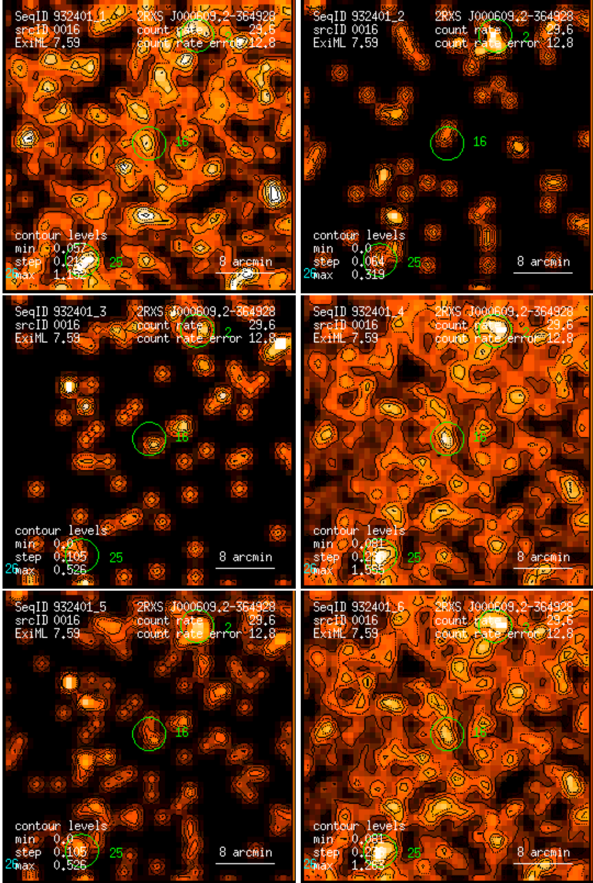
Figure 16: RASS 932401: detection 0016: band rate images, Gaussian filter: (1) PSPC channels 11 – 41, (2) 52 – 90, (3) 91 – 201, (4) 11 – 235, (5) 52 – 201, (6) 11 – 201. Broad band rates in counts/ks. Band rate contour levels in counts/ks/arcmin 2 .
