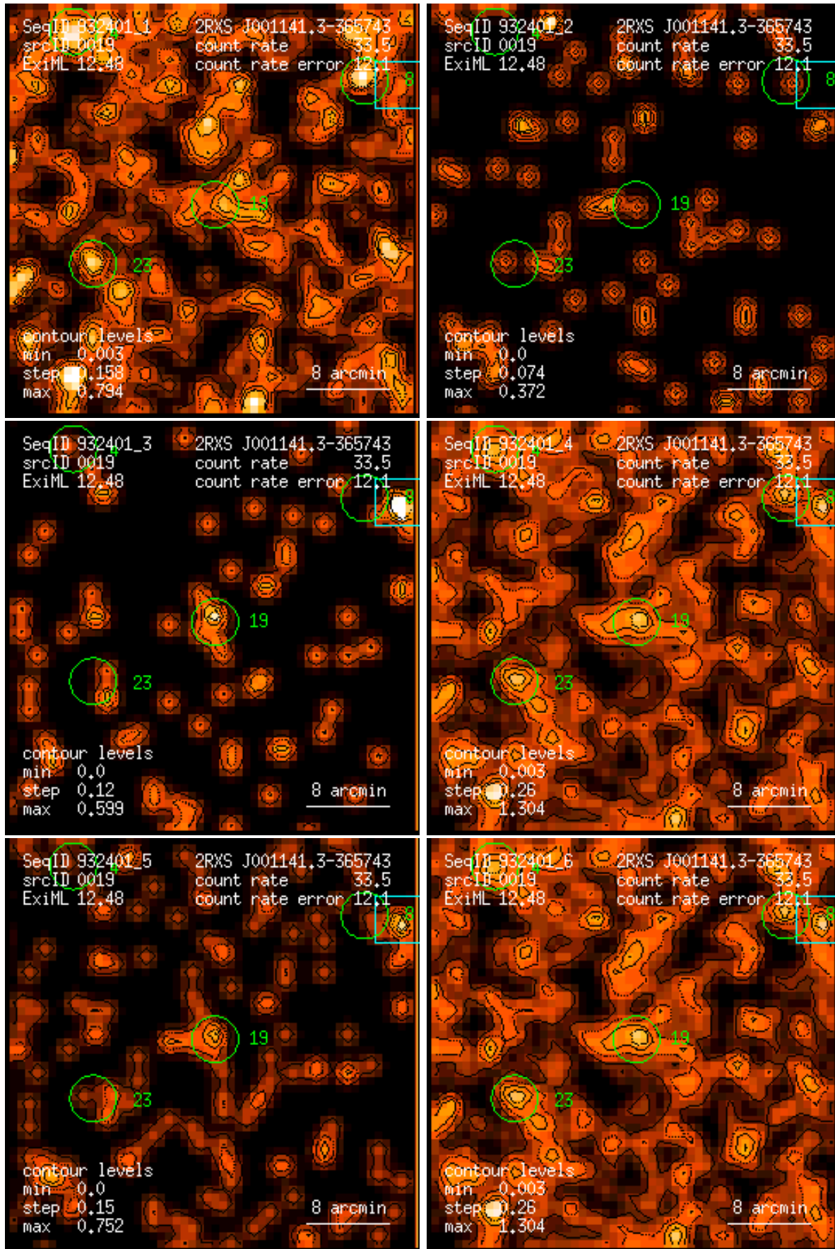
Figure 19: RASS 932401: detection 0019: band rate images, Gaussian filter: (1) PSPC channels 11 – 41, (2) 52 – 90, (3) 91 – 201, (4) 11 – 235, (5) 52 – 201, (6) 11 – 201. Broad band rates in counts/ks. Band rate contour levels in counts/ks/arcmin 2 .
