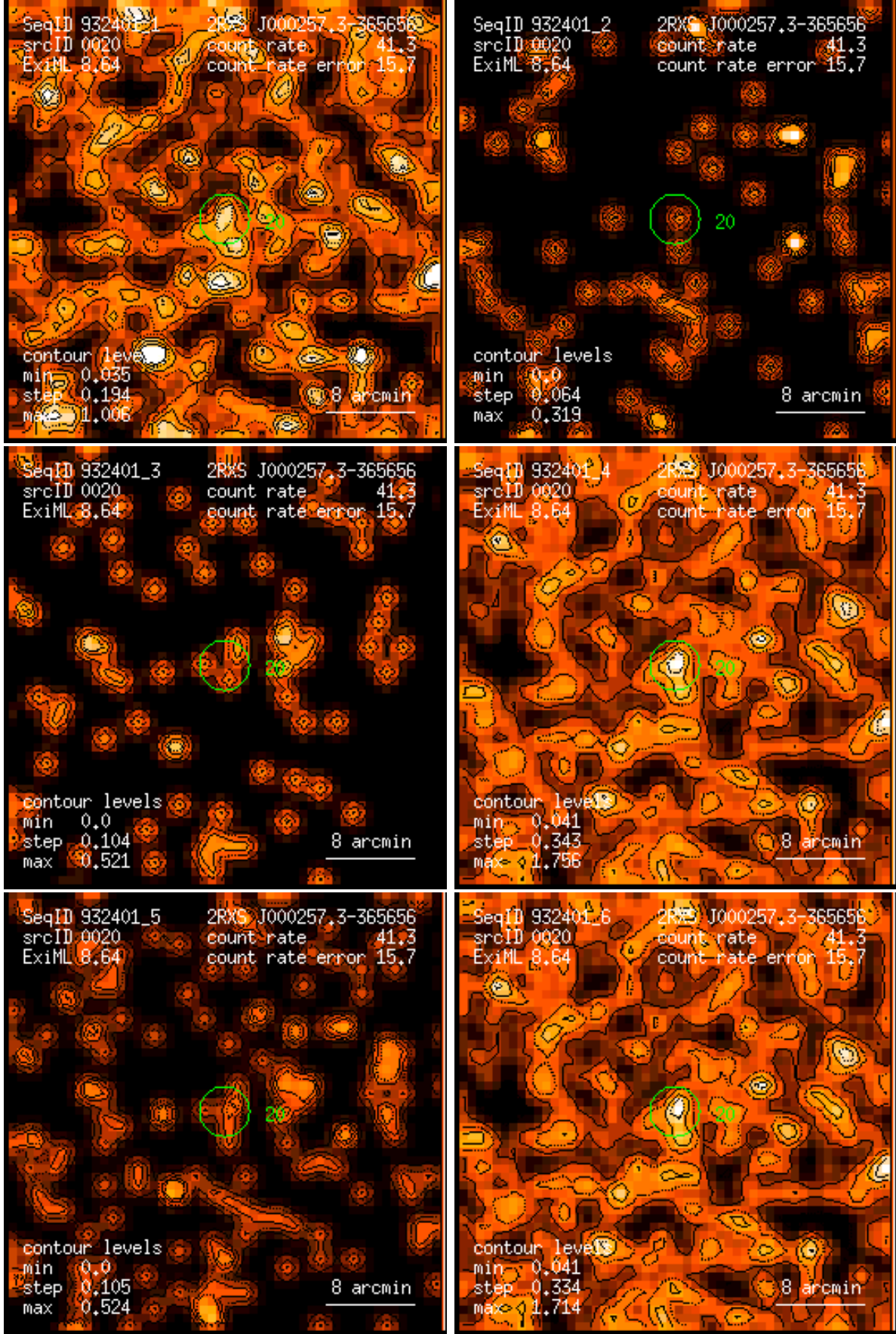
Figure 20: RASS 932401: detection 0020: band rate images, Gaussian filter: (1) PSPC channels 11 – 41, (2) 52 – 90, (3) 91 – 201, (4) 11 – 235, (5) 52 – 201, (6) 11 – 201. Broad band rates in counts/ks. Band rate contour levels in counts/ks/arcmin 2 .
