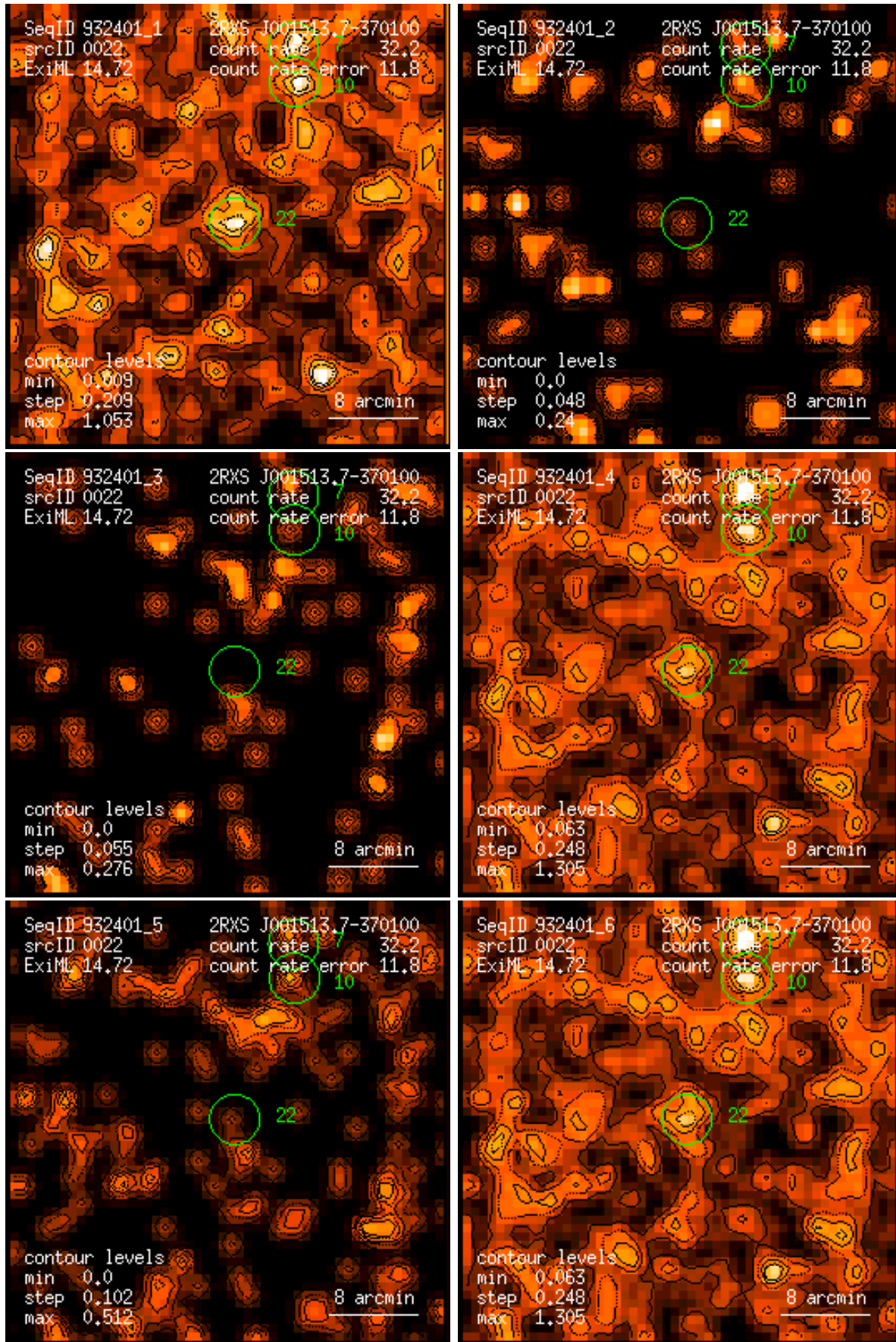
Figure 22: RASS 932401: detection 0022: band rate images, Gaussian filter: (1) PSPC channels 11 – 41, (2) 52 – 90, (3) 91 – 201, (4) 11 – 235, (5) 52 – 201, (6) 11 – 201. Broad band rates in counts/ks. Band rate contour levels in counts/ks/arcmin 2 .
