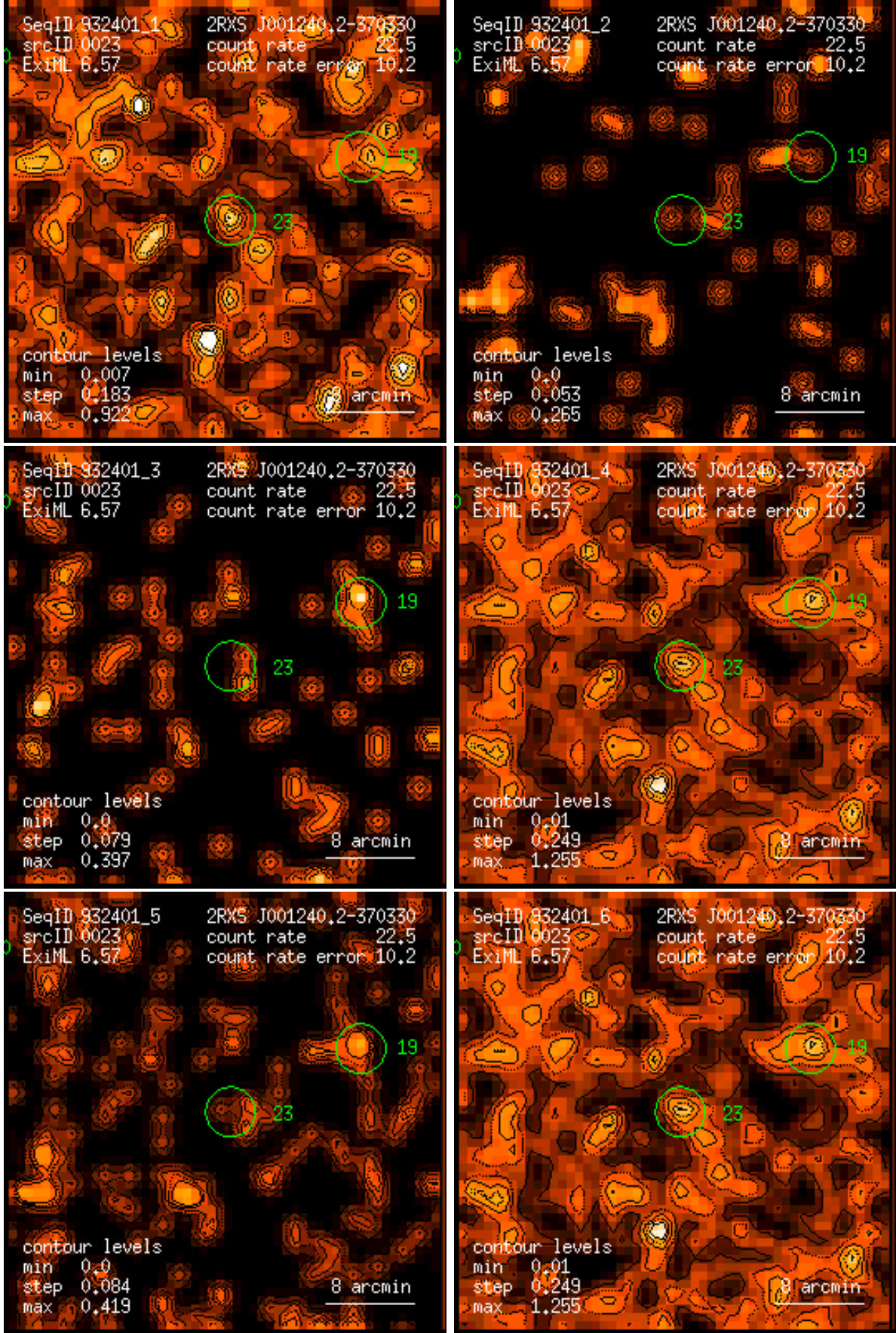
Figure 23: RASS 932401: detection 0023: band rate images, Gaussian filter: (1) PSPC channels 11 – 41, (2) 52 – 90, (3) 91 – 201, (4) 11 – 235, (5) 52 – 201, (6) 11 – 201. Broad band rates in counts/ks. Band rate contour levels in counts/ks/arcmin 2 .
