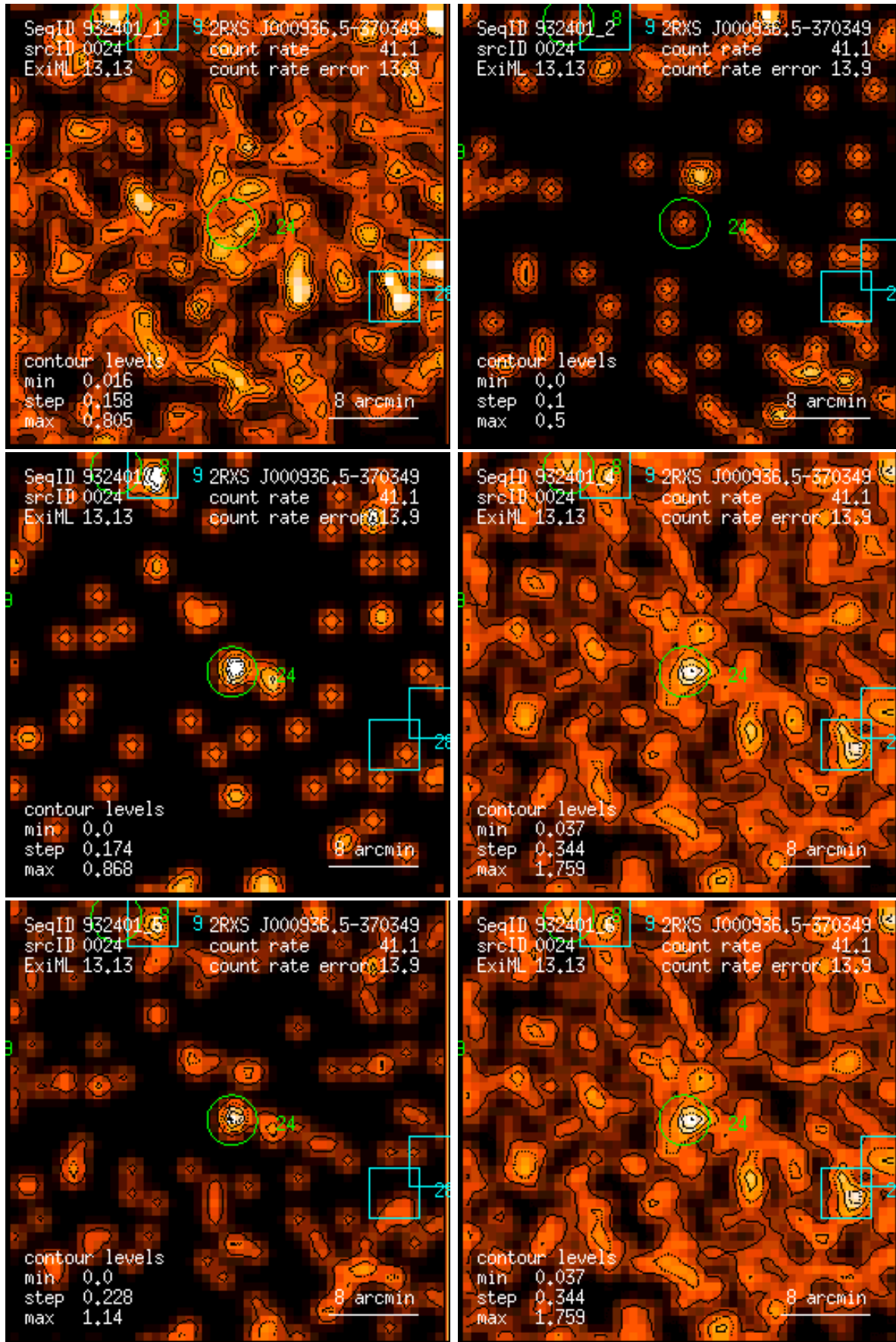
Figure 24: RASS 932401: detection 0024: band rate images, Gaussian filter: (1) PSPC channels 11 – 41, (2) 52 – 90, (3) 91 – 201, (4) 11 – 235, (5) 52 – 201, (6) 11 – 201. Broad band rates in counts/ks. Band rate contour levels in counts/ks/arcmin 2 .
