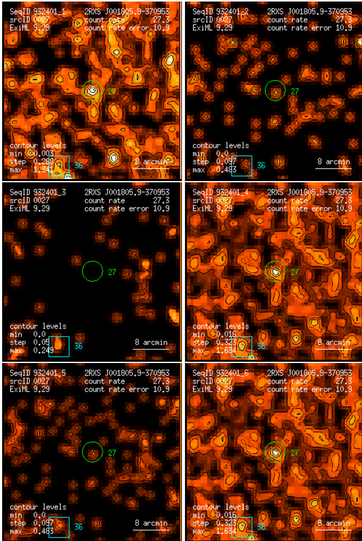
Figure 27: RASS 932401: detection 0027: band rate images, Gaussian filter: (1) PSPC channels 11 – 41, (2) 52 – 90, (3) 91 – 201, (4) 11 – 235, (5) 52 – 201, (6) 11 – 201. Broad band rates in counts/ks. Band rate contour levels in counts/ks/arcmin 2 .
