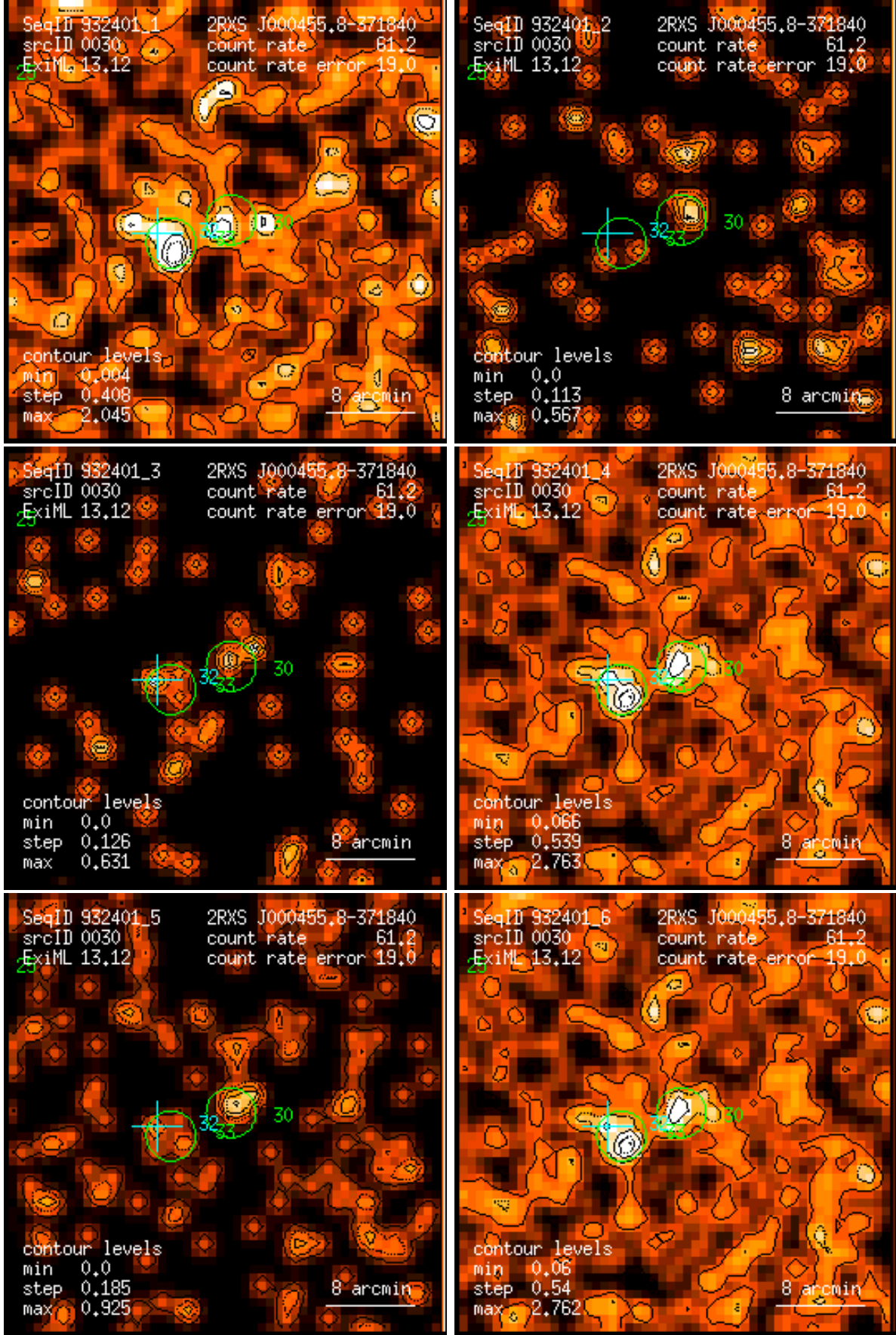
Figure 30: RASS 932401: detection 0030: band rate images, Gaussian filter: (1) PSPC channels 11 – 41, (2) 52 – 90, (3) 91 – 201, (4) 11 – 235, (5) 52 – 201, (6) 11 – 201. Broad band rates in counts/ks. Band rate contour levels in counts/ks/arcmin 2 .
