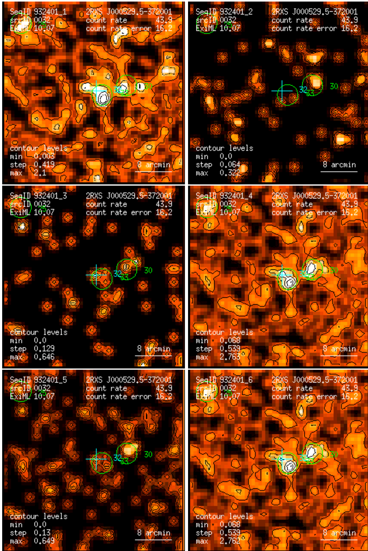
Figure 32: RASS 932401: detection 0032: band rate images, Gaussian filter: (1) PSPC channels 11 – 41, (2) 52 – 90, (3) 91 – 201, (4) 11 – 235, (5) 52 – 201, (6) 11 – 201. Broad band rates in counts/ks. Band rate contour levels in counts/ks/arcmin 2 .
