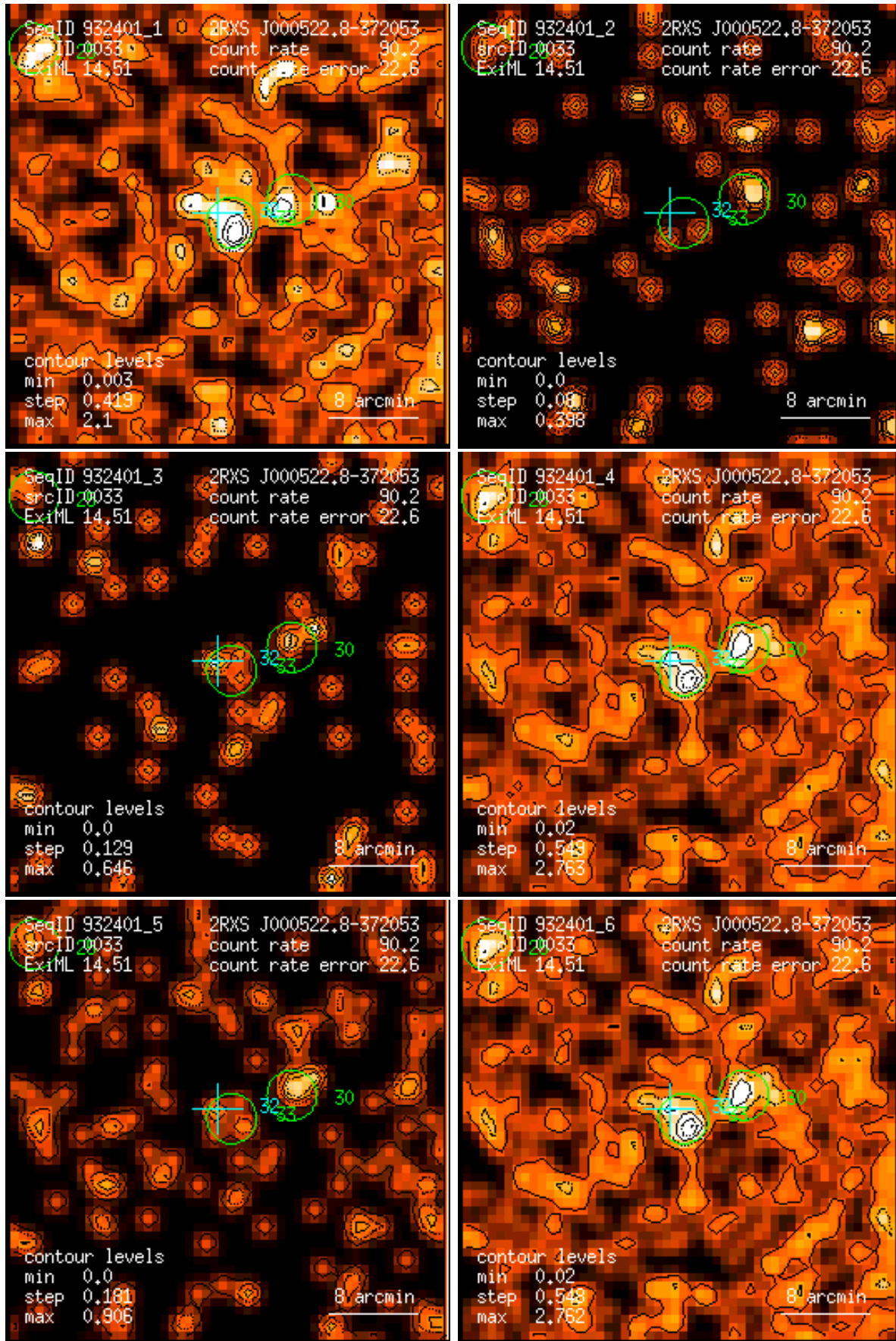
Figure 33: RASS 932401: detection 0033: band rate images, Gaussian filter: (1) PSPC channels 11 – 41, (2) 52 – 90, (3) 91 – 201, (4) 11 – 235, (5) 52 – 201, (6) 11 – 201. Broad band rates in counts/ks. Band rate contour levels in counts/ks/arcmin 2 .
